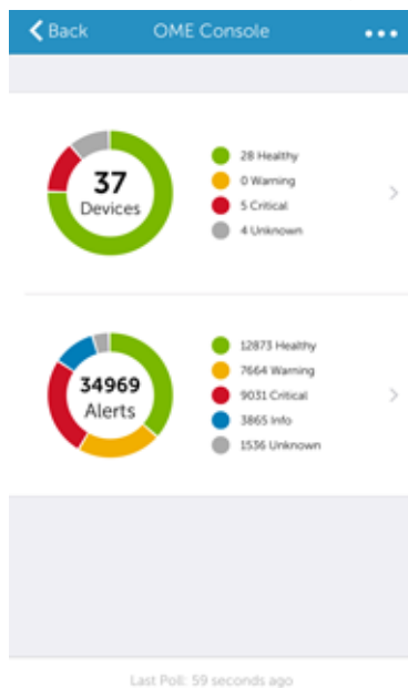
Figure 6. OME dashboard
