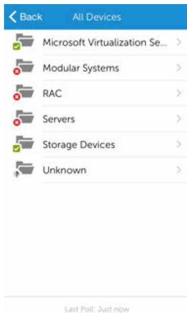
Figure 7. All devices
