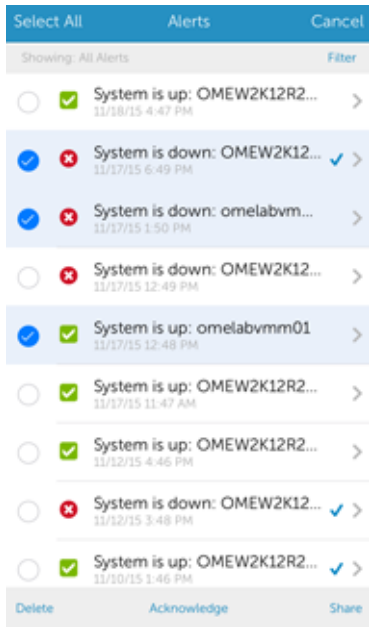
Figure 12. Deleting alerts
