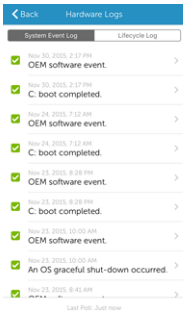
Figure 18. Hardware logs
