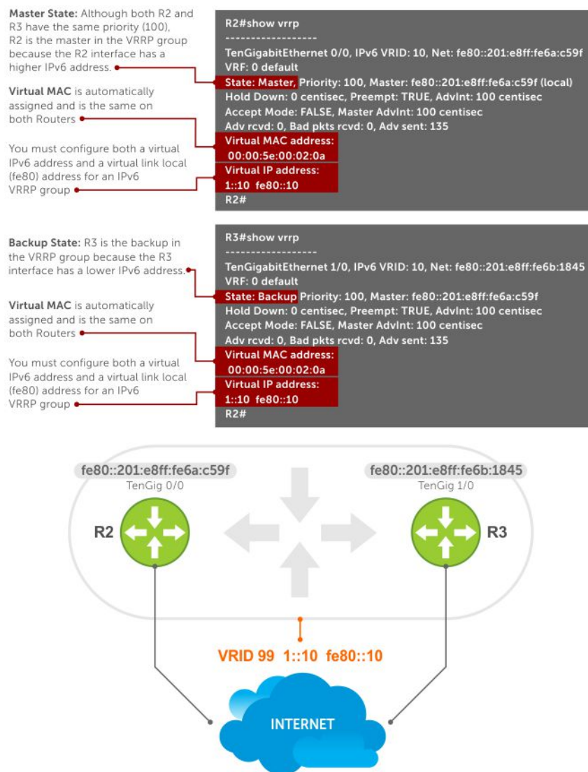
Figure 164. VRRP for IPv6 Topology
