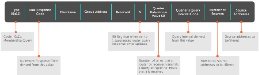
Figure 44. IGMP Version 3 Packet Structure
