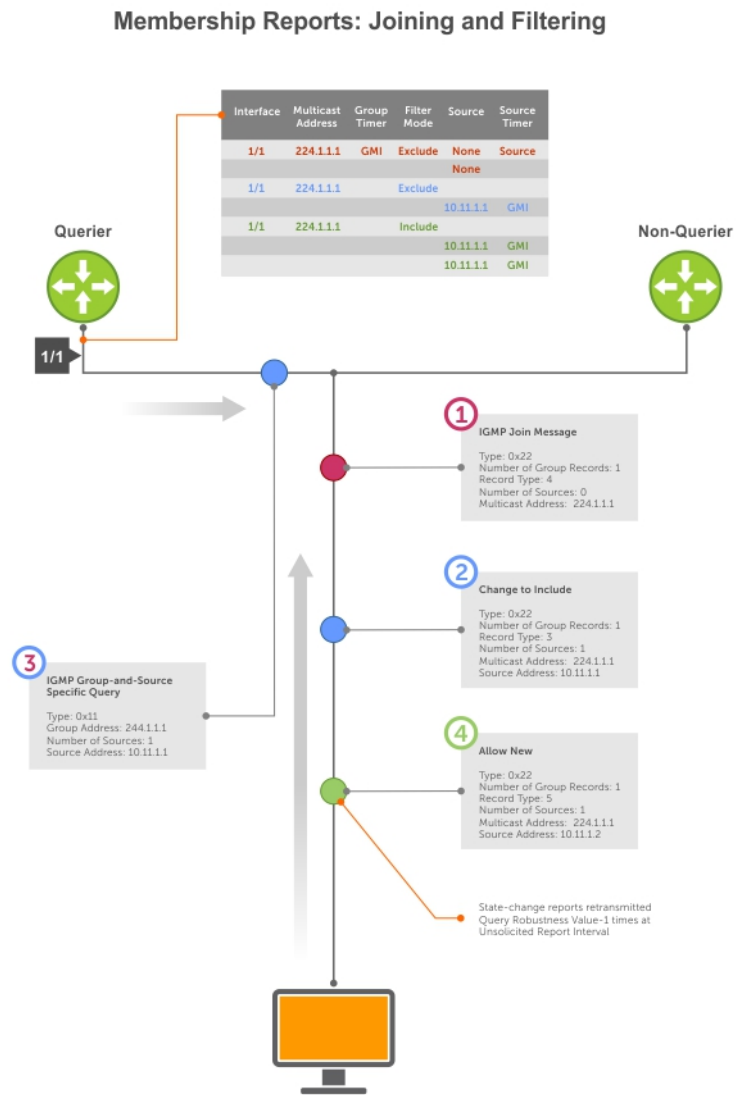
Figure 37. Membership Reports: Joining and Filtering
