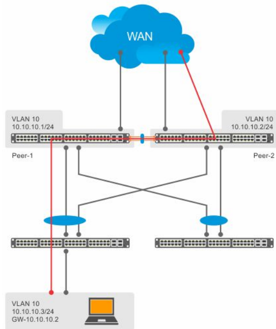
Figure 133. Packets without peer routing enabled
