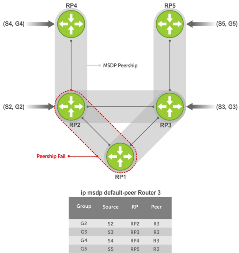
Figure 81. MSDP Default Peer, Scenario 3
