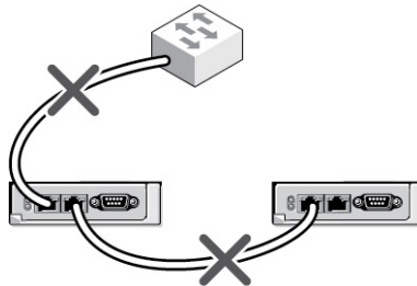
Figure 4. Incorrect cabling for CMC network — single CMC
