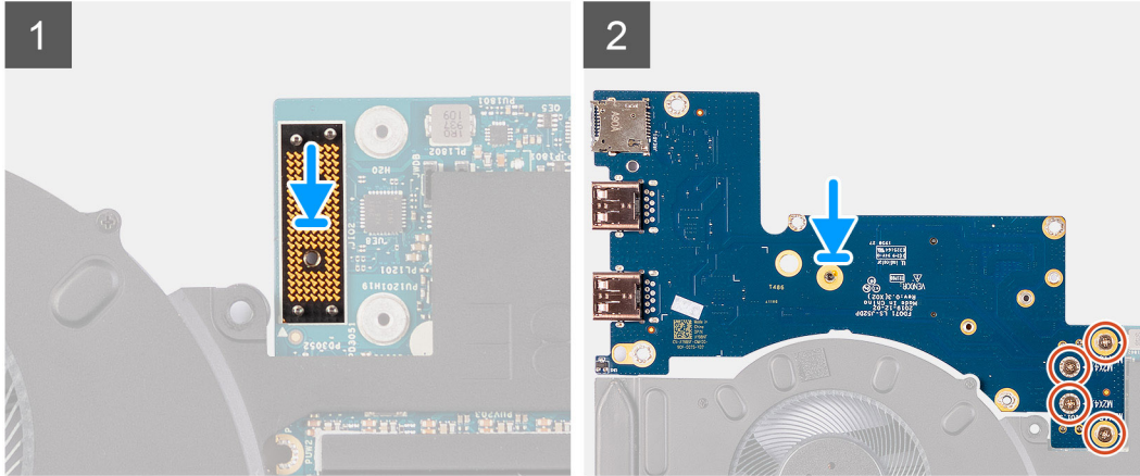
4x M2x4.5
