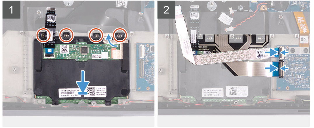
4x M2x2.5
