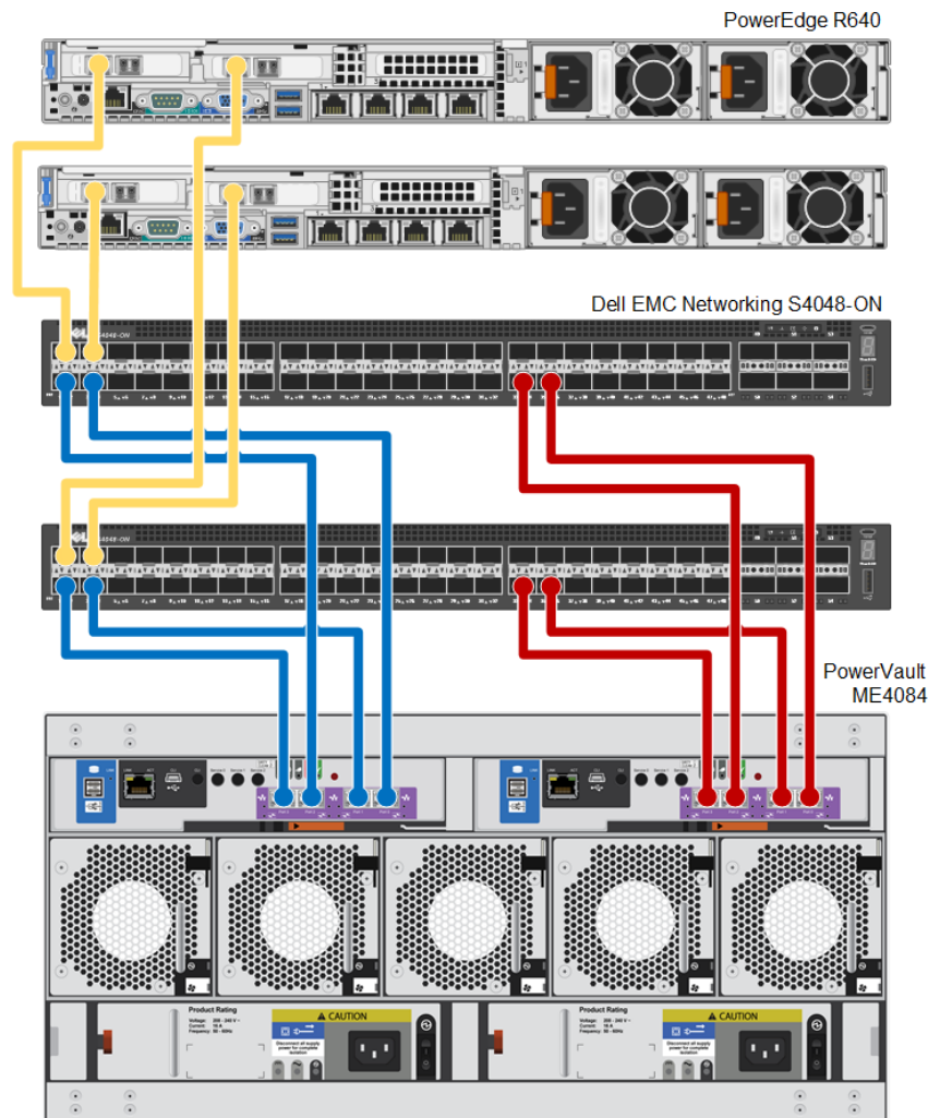
Figure 2 Connecting two hosts to an ME4084 array using two switches
