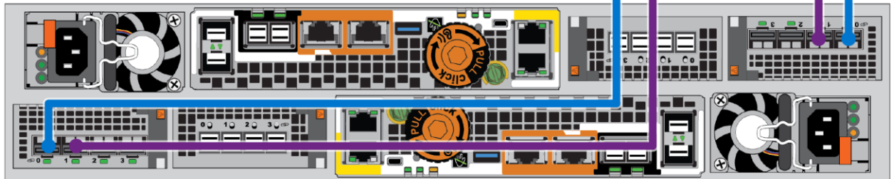
Figure 2 Dell EMC Unity cabling diagram
