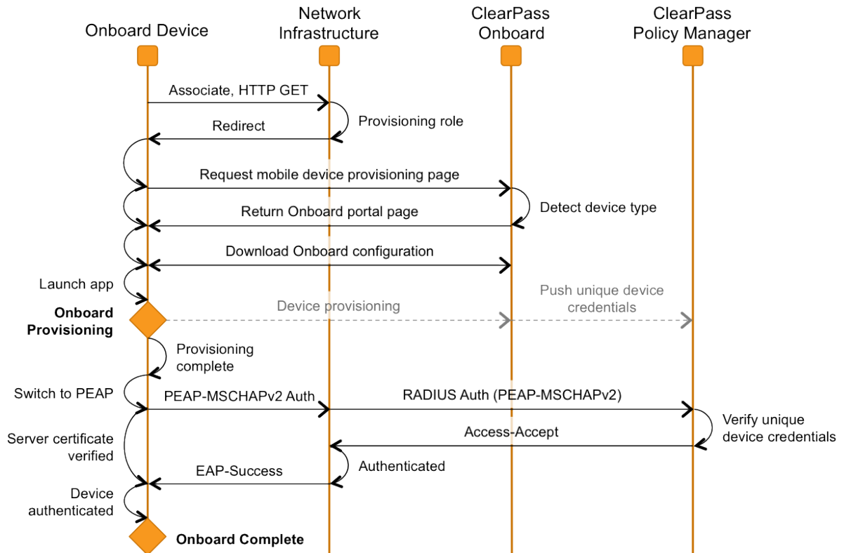
Figure 19 Sequence Diagram for the Onboard Workflow on Android Platform
