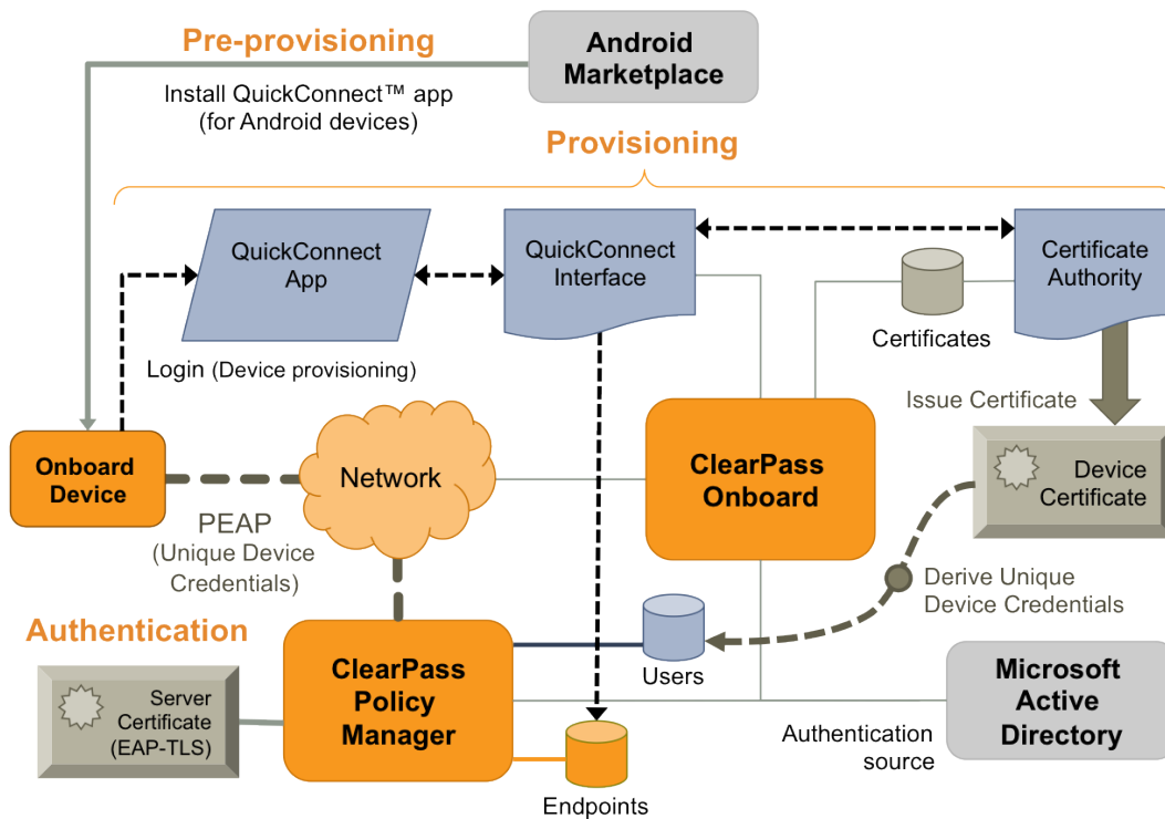
Figure 18 W-ClearPass Onboard Process for Onboard-Capable Devices
