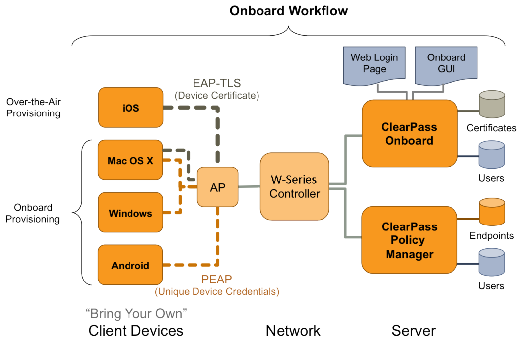
Figure 13 Detailed View of the W-ClearPass Onboard Network Architecture
