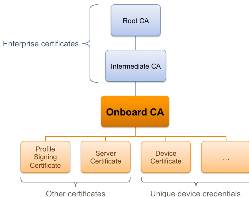
Figure 11 Relationship of Certificates in the Onboard Public Key Infrastructure
