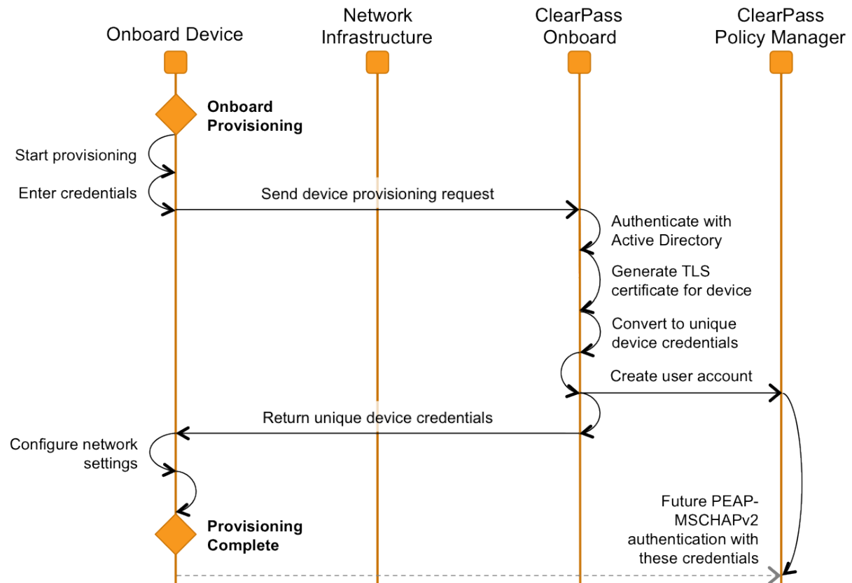
Figure 20 Onboard Provisioning Workflow in the QuickConnect App
