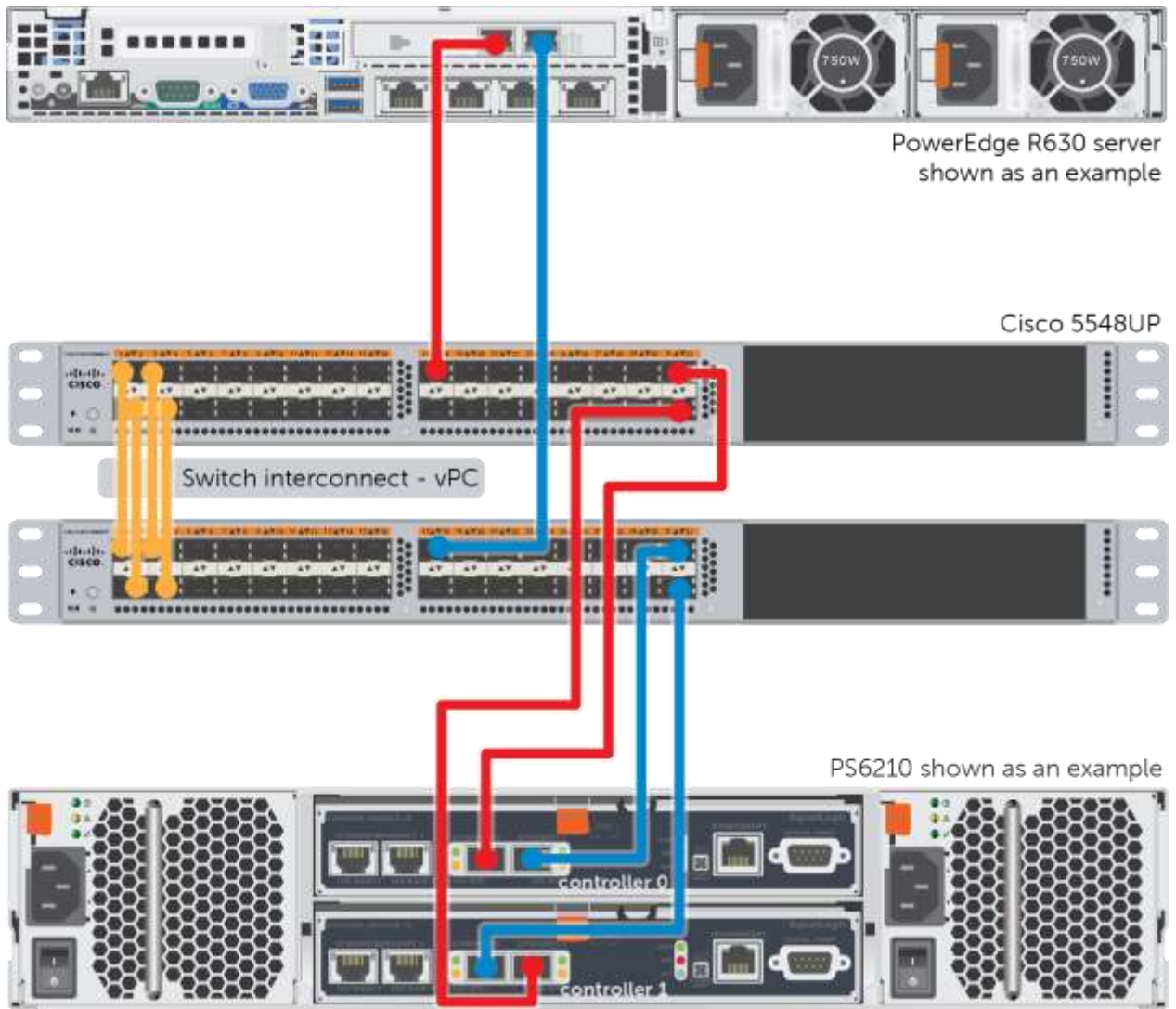
Figure 1 Cabling diagram
