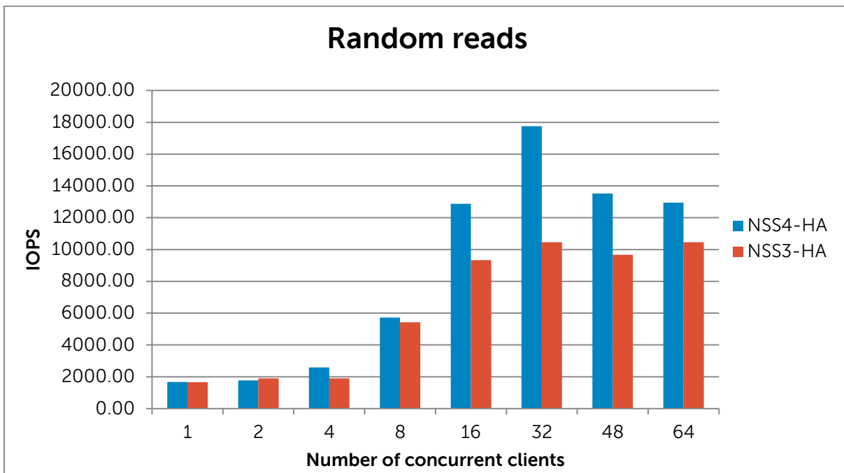
Figure 8. IPoB random read performance: NSS4-HA vs. NSS3-HA
