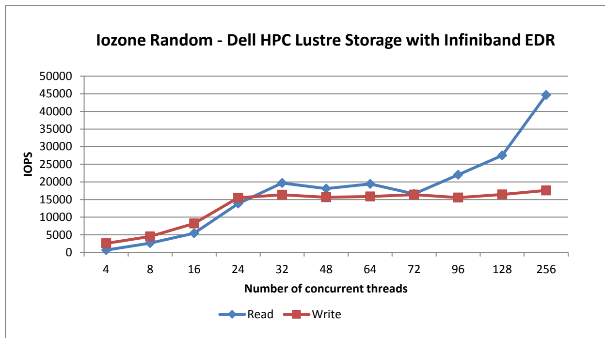
Figure 11: N-to-N Random reads and writes
