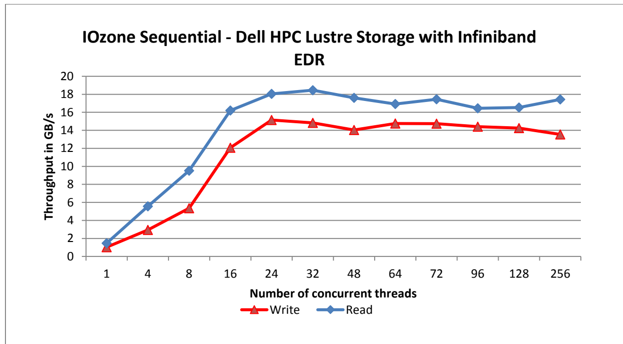
Figure 10: Sequential Reads / Writes Dell HPC Lustre Storage with Infiniband EDR
