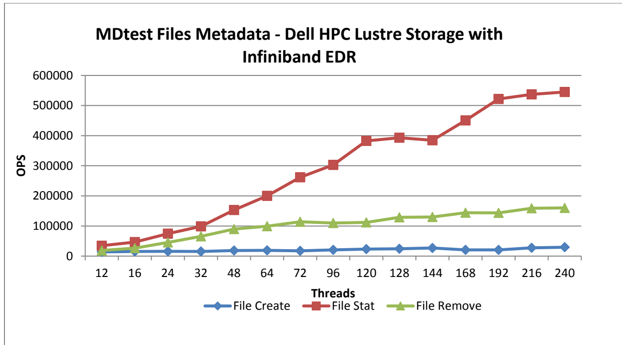
Figure 12: File Metadata Operations
