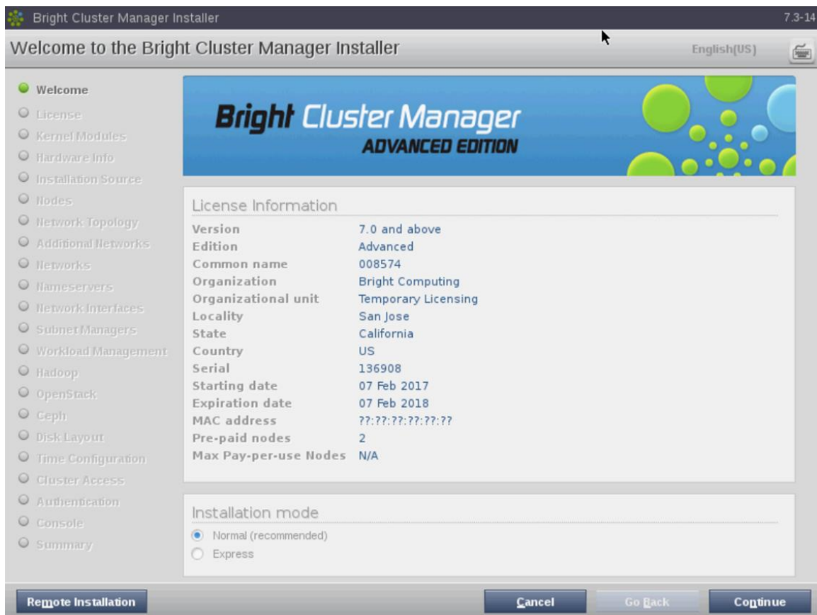
Figure 4 Welcome screen
