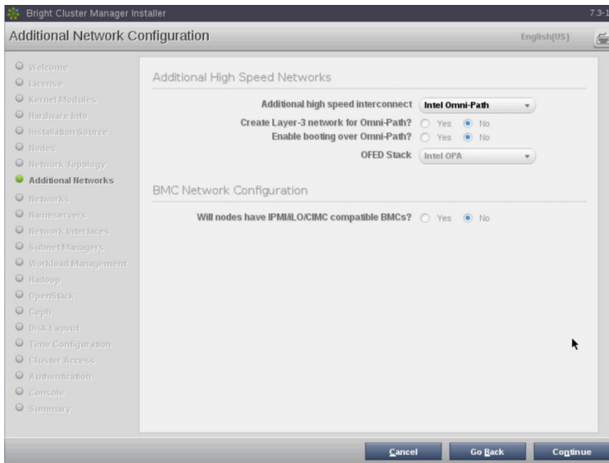
Figure 6 Intel Omni-Path Setup
