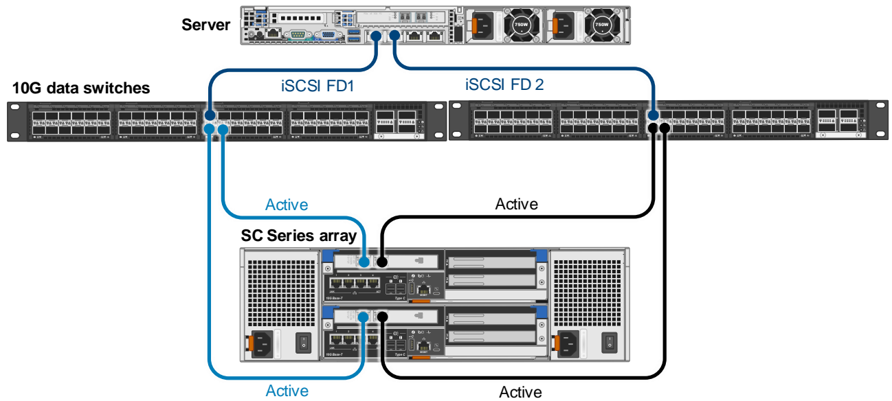
Figure 3 Virtual port mode cabling example with iSCSI
