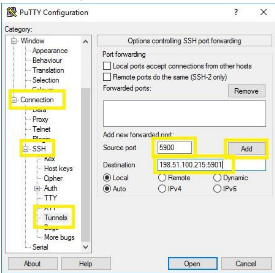
Figure 11 Configuring PuTTY
