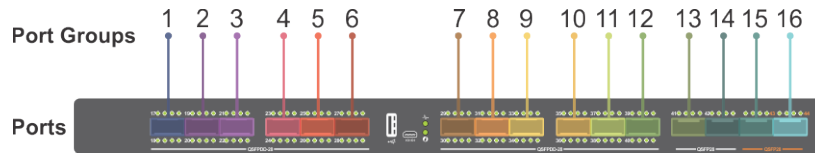
Figure 6. MX9116n Fabric Switching Engine unified port groups
