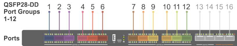
Figure 1. MX9116n Fabric Switching Engine — QSFP28-DD port groups
