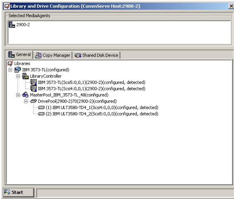
14: CommVault
