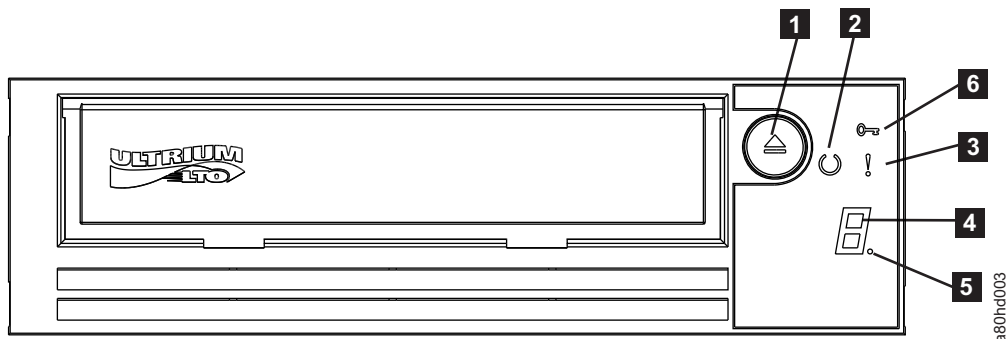
Figure 1-4. Front Panel
