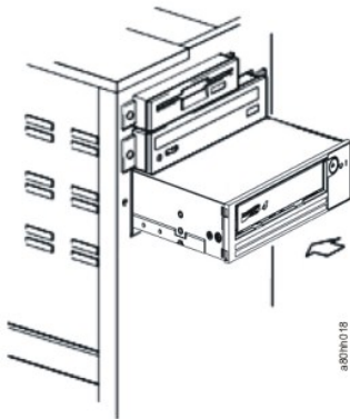
Figure 7. Install the Drive
