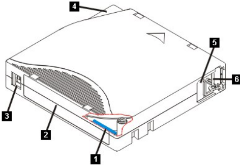
Figure 14. LTO Ultrium 800 GB Data Cartridge
