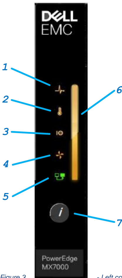
Figure 3 - Left control panel (Status LED Version)
