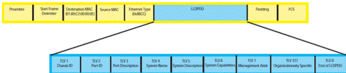
Figure 65. LLDPDU Frame
