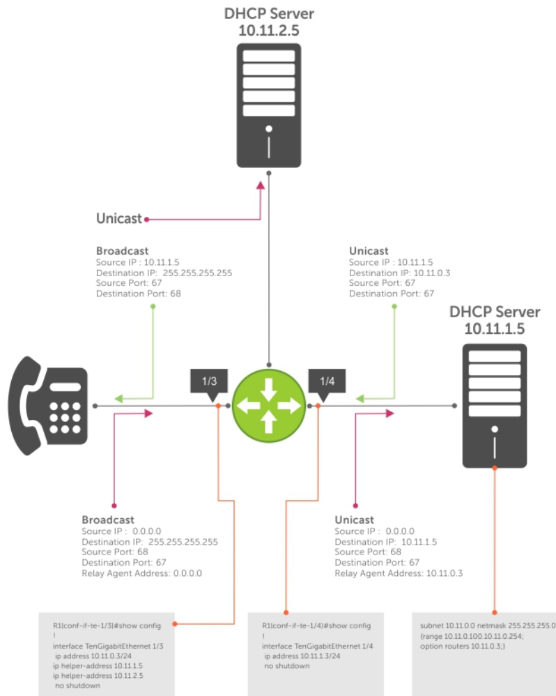
Figure 31. Assigning Network Parameters using DHCP
