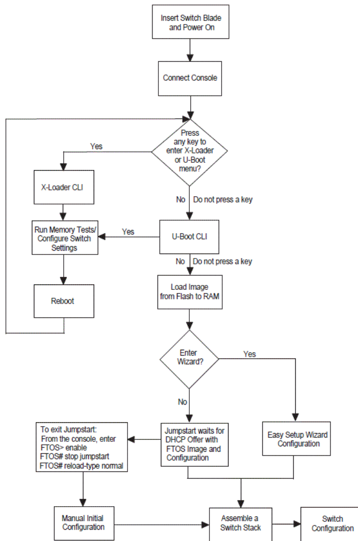
Figure 129. Installing and Configuring Flowchart for FC Flex IO Modules
