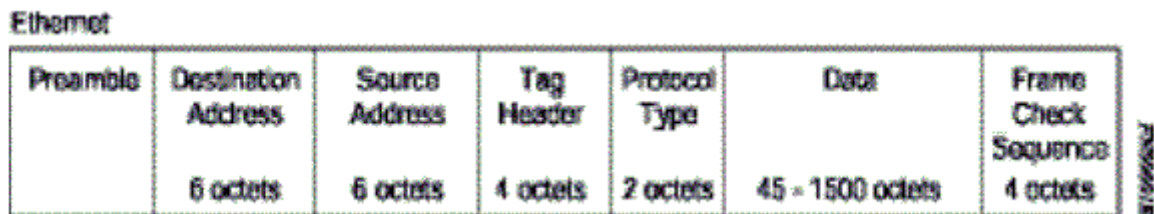
Figure 50. Tagged Frame Format
