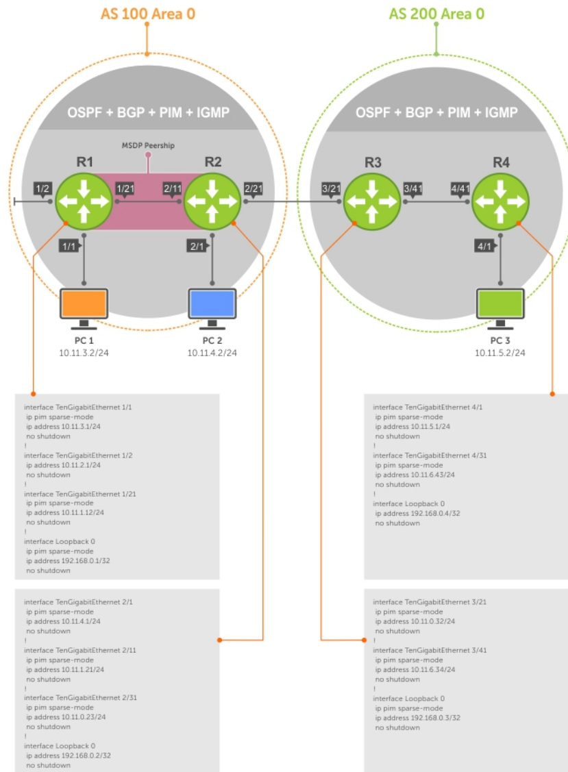
Figure 72. Multicast Source Discovery Protocol (MSDP)
