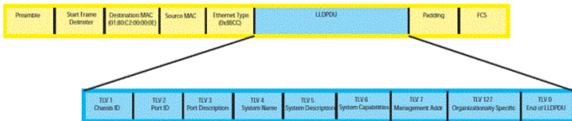
Figure 65. LLDPDU Frame
