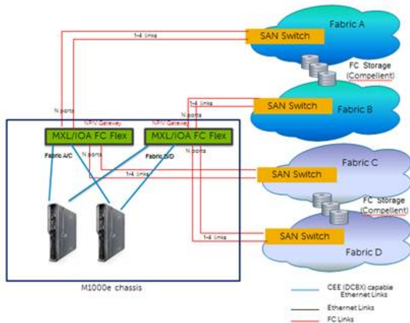
Figure 130. Case 1: Deployment Scenario of Configuring FC Flex IO Modules
