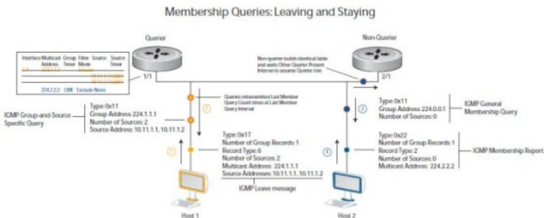
Figure 49. IGMP Membership Queries: Leaving and Staying in Groups
