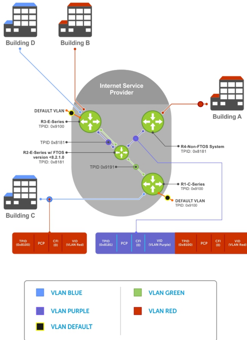
Figure 107. Single and Double-Tag TPID Mismatch
