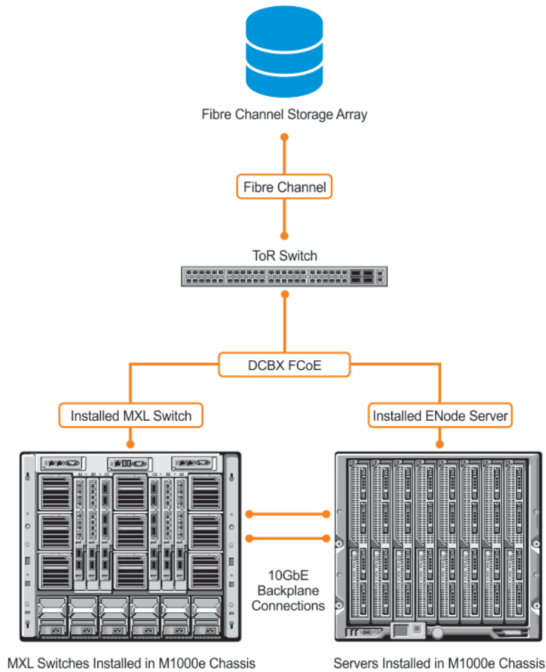
Figure 35. FIP Snooping on an FN IOMSwitch Configuration Example
