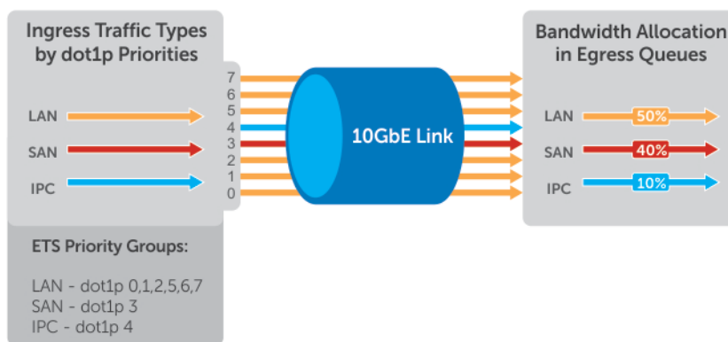
Figure 133. Enhanced Transmission Selection
