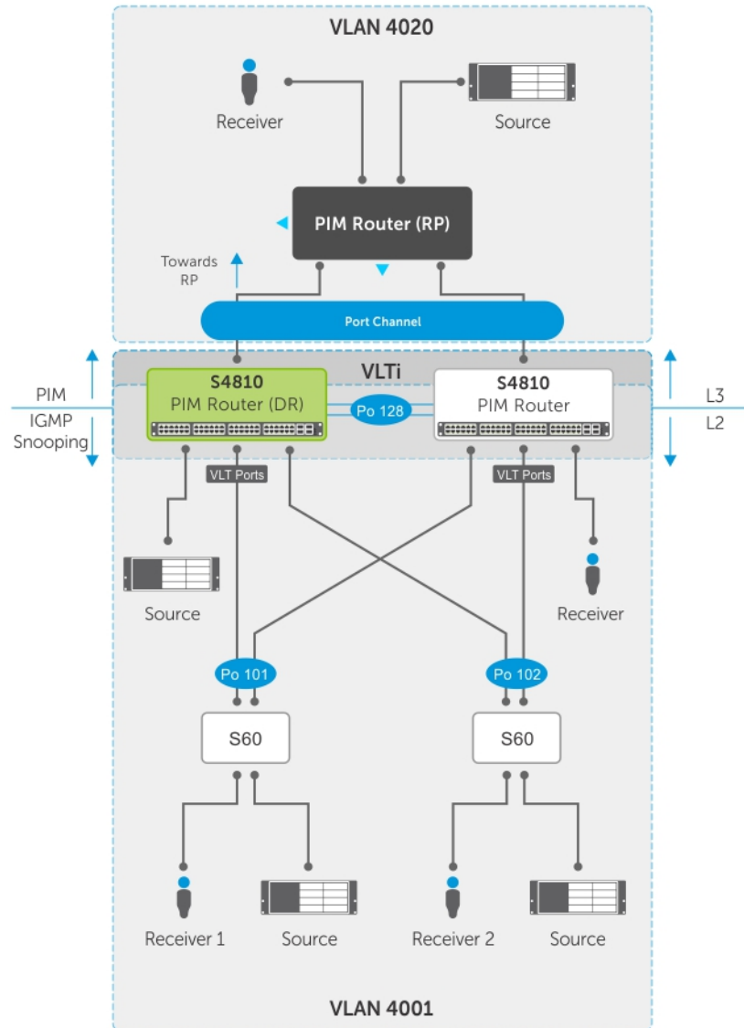
Figure 125. PIM-Sparse Mode Support on VLT
