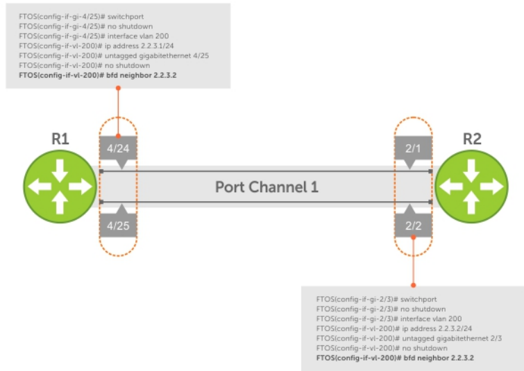
Figure 16. Establishing Sessions on Port-Channels
