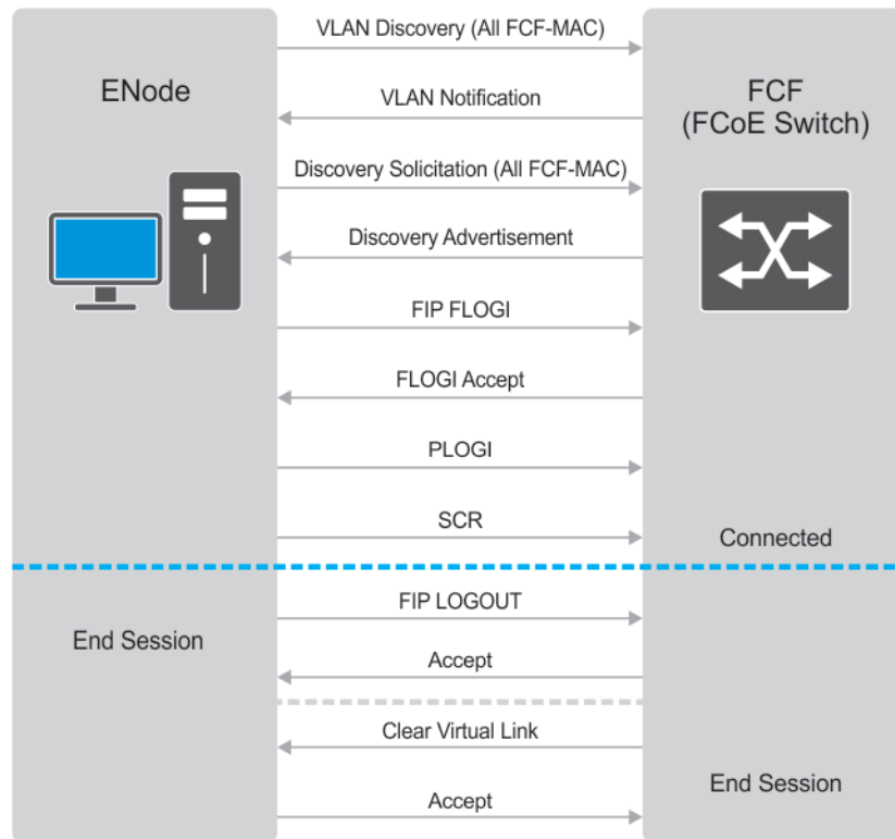
Figure 33. FIP Discovery and Login Between an ENode and an FCF
