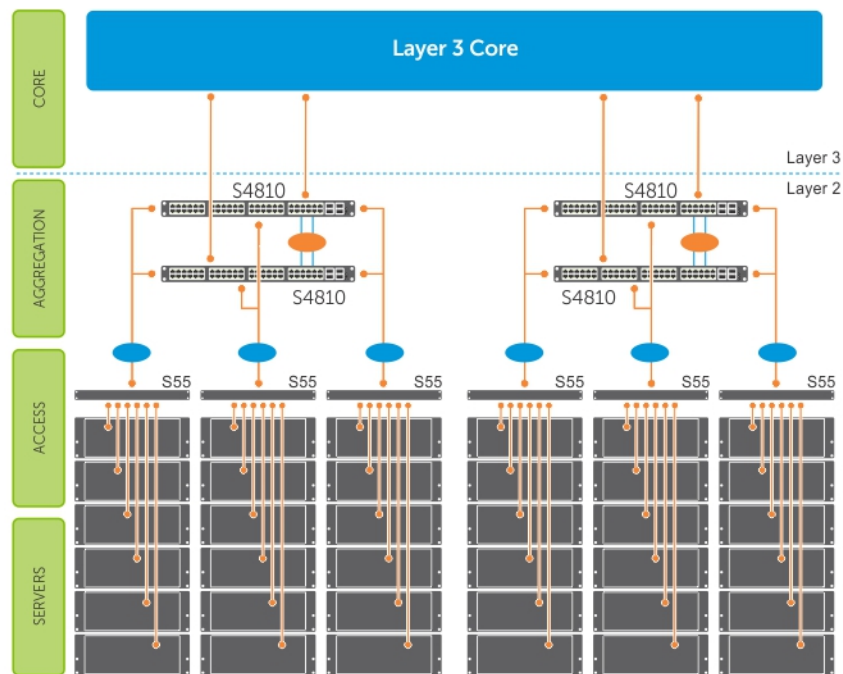
Figure 124. Multi-Domain VLT Example
