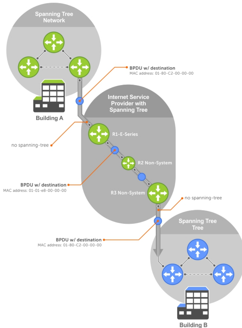
Figure 110. VLAN Stacking with L2PT
