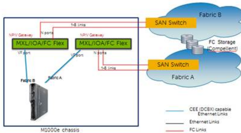
Figure 131. Case 2: Deployment Scenario of Configuring FC Flex IO Modules
