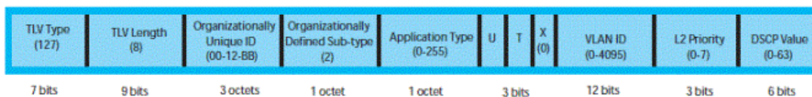
Figure 69. LLDP-MED Policies TLV
