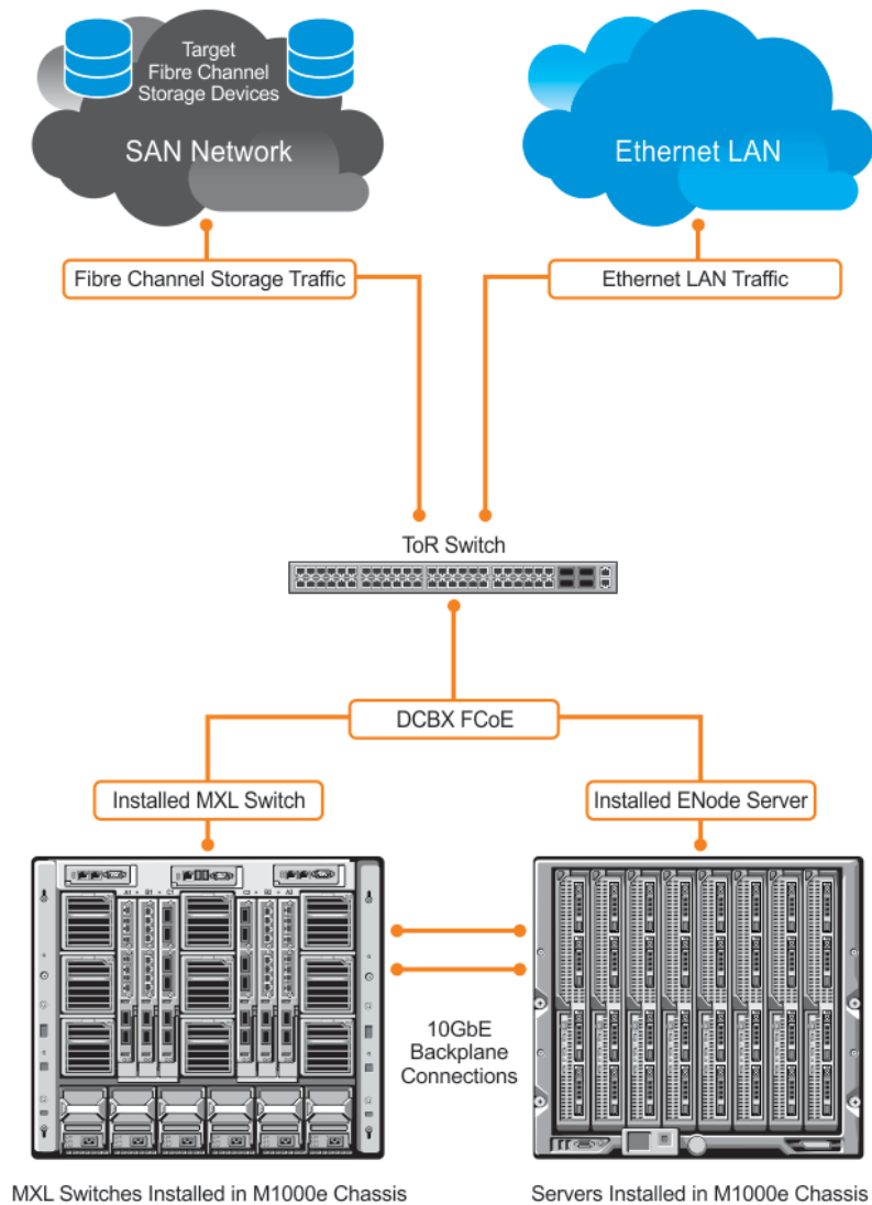
Figure 34. FIP Snooping on an FN IOM Switch
