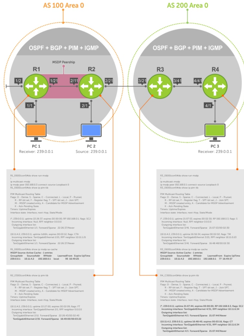
Figure 74. Configuring Interfaces for MSDP
