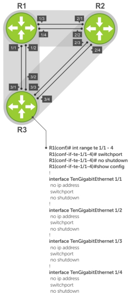
Figure 111. Example of Configuring Interfaces for Layer 2 Mode
