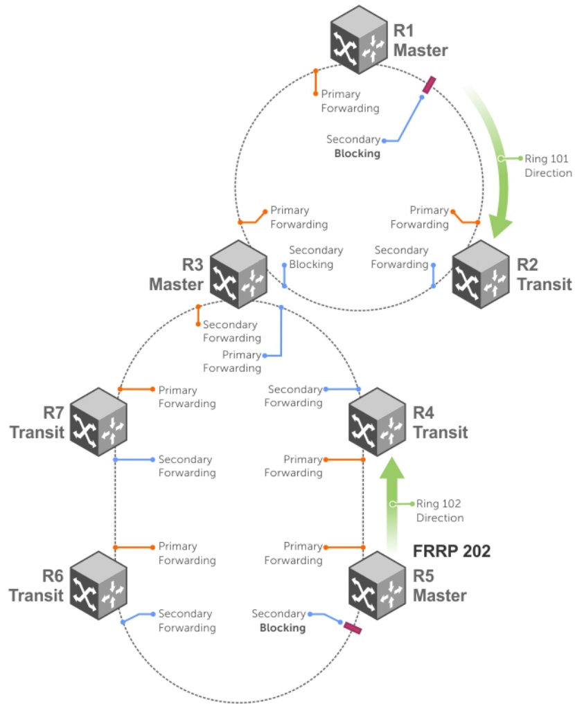
Figure 37. Multiple Rings Connected by a Single Switch Example
