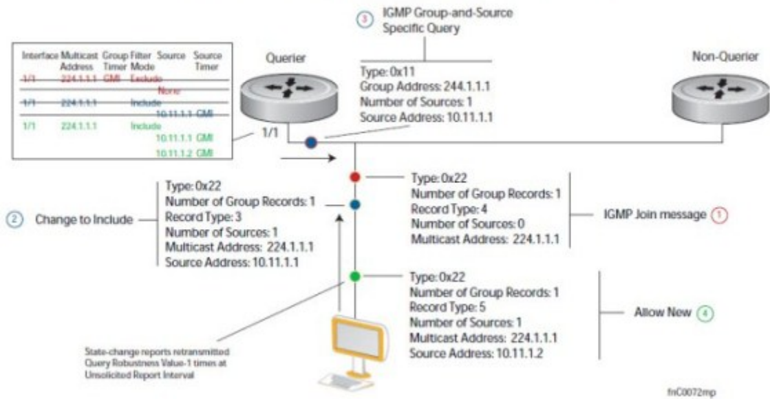
Figure 48. IGMP Membership Reports: Joining and Filtering
