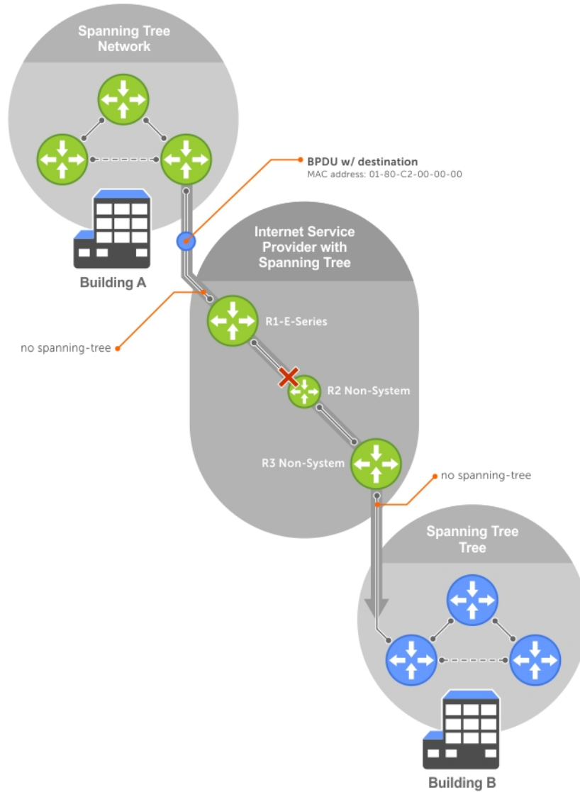
Figure 109. VLAN Stacking without L2PT
