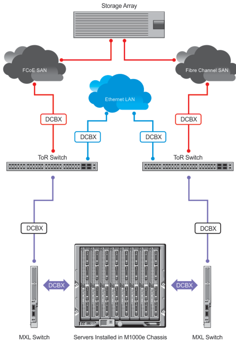
Figure 136. PFC and ETS Applied to LAN, IPC, and SAN Priority Traffic
