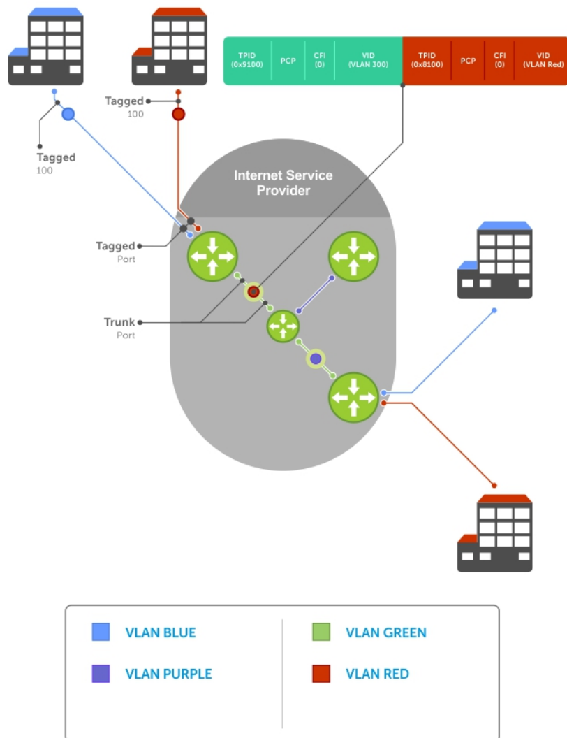
Figure 104. VLAN Stacking in a Service Provider Network
