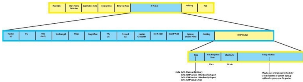
Figure 45. IGMP Version 2 Packet Format
