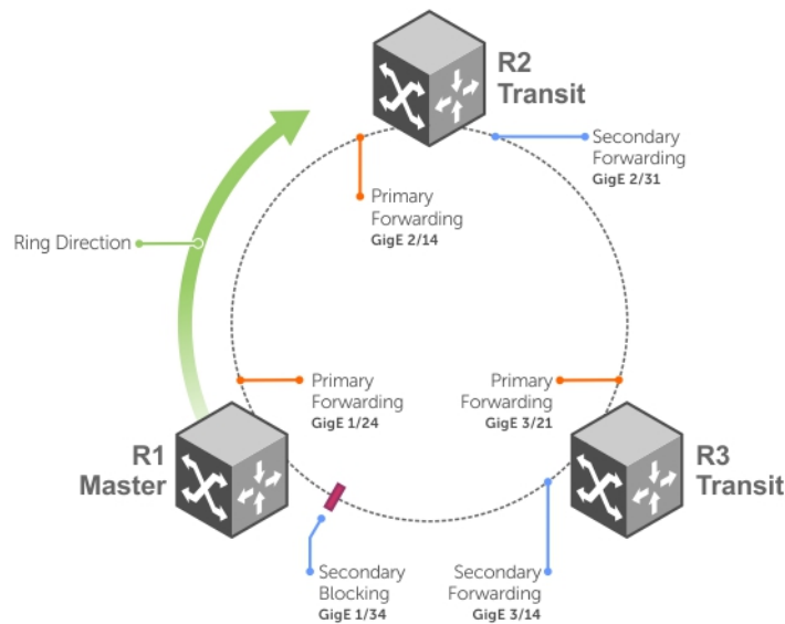
Figure 38. Basic Topology and CLI Commands
