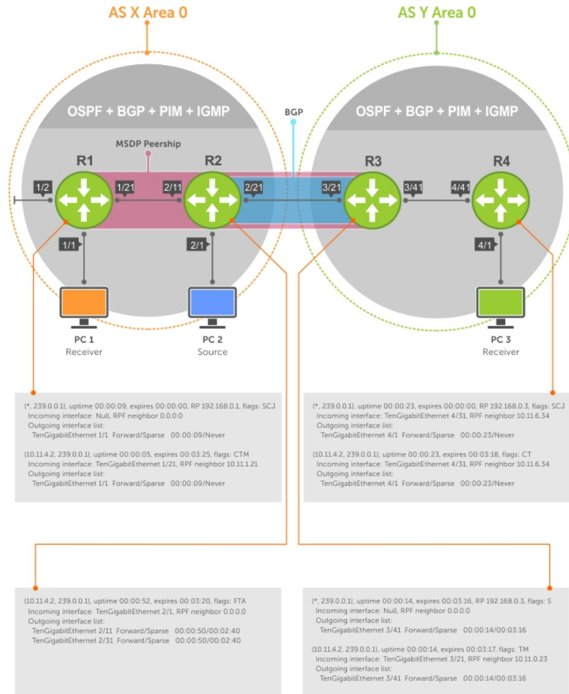
Figure 75. Configuring OSPF and BGP for MSDP
