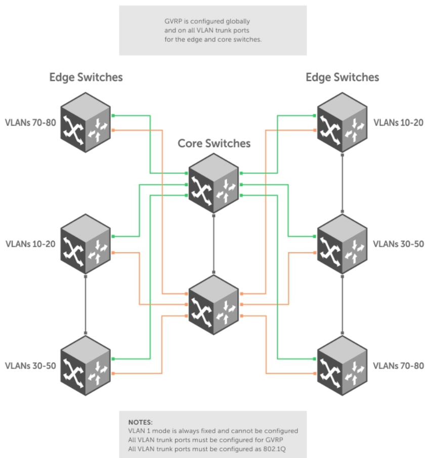
Figure 41. Global GVRP Configuration Example
