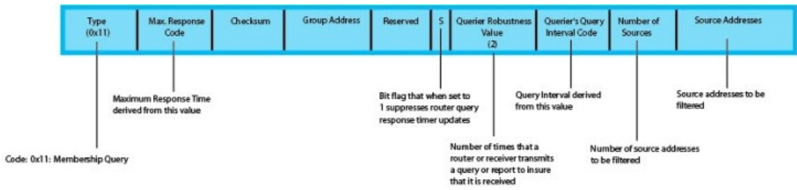
Figure 46. IGMP version 3 Membership Query Packet Format
