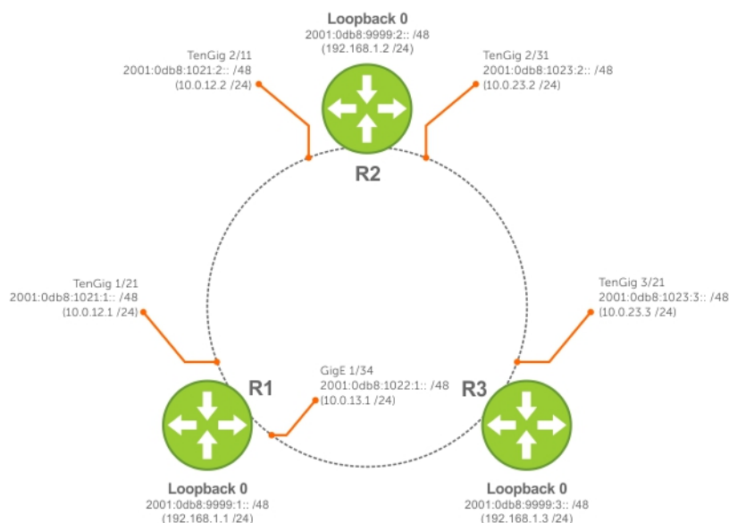
Figure 61. IPv6 IS-IS Sample Topography
