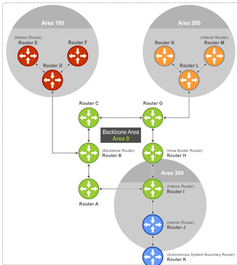
Figure 88. Autonomous System Areas
