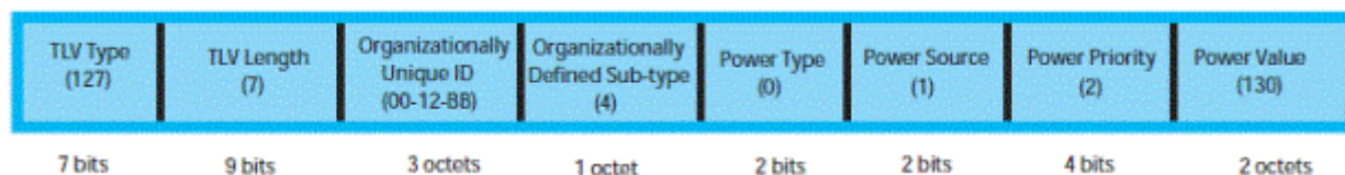
Figure 70. Extended Power via MDI TLV
