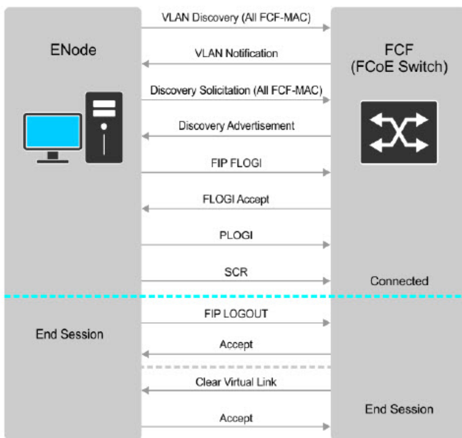
Figure 42. FIP Discovery and Login between an ENode and an FCF
