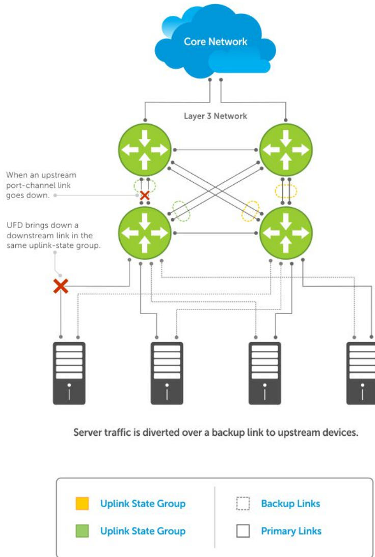
Figure 120. Uplink Failure Detection Example
