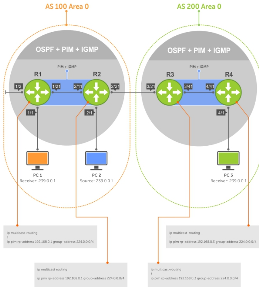
Figure 76. Configuring PIM in Multiple Routing Domains
