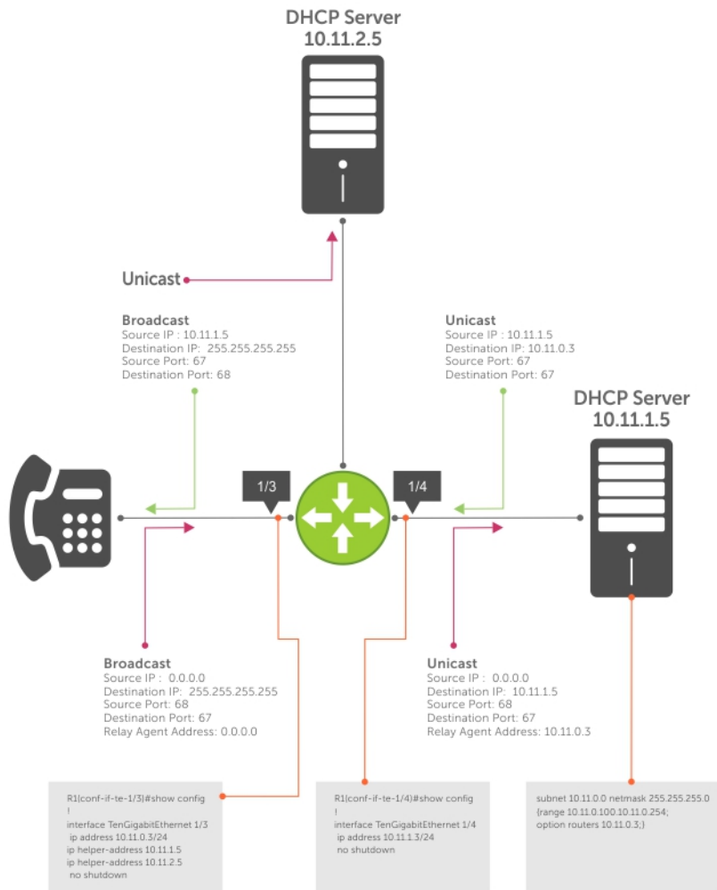
Figure 31. Assigning Network Parameters using DHCP
