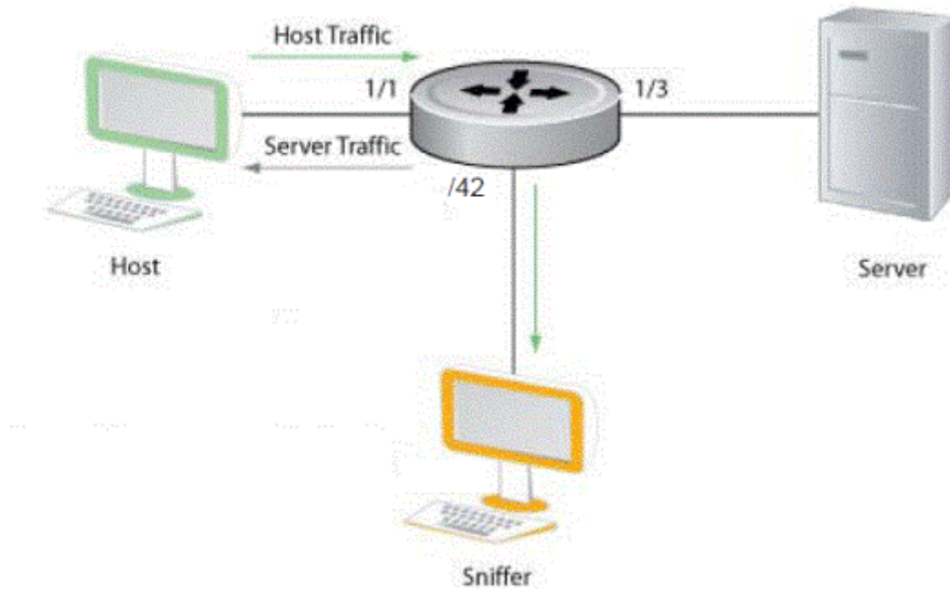
Figure 92. Port Monitoring Example
