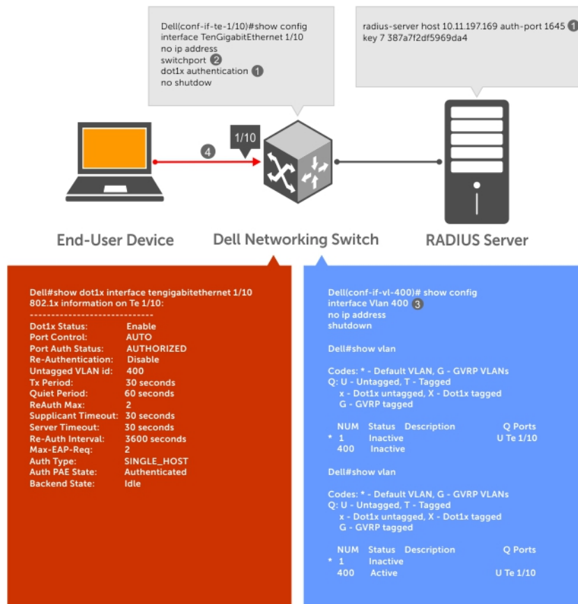
Figure 4. EAP Port-Authentication
