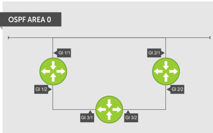
Figure 91. Basic Topology and CLI Commands for OSPFv2
