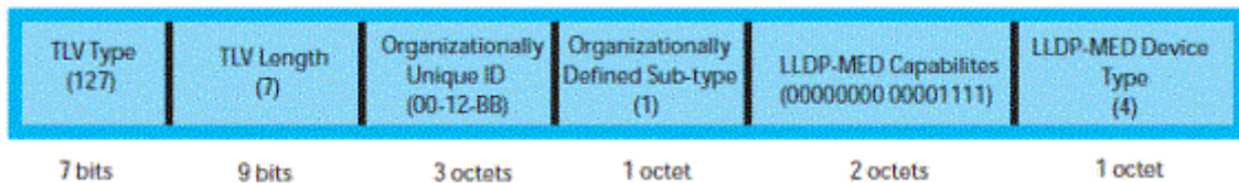
Figure 68. LLDP-MED Capabilities TLV
