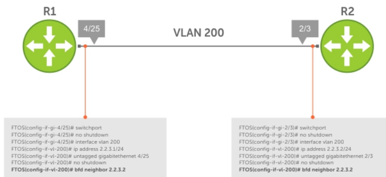
Figure 15. Establishing Sessions with VLAN Neighbors
