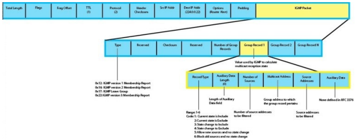
Figure 47. IGMP version 3 Membership Report Packet Format
