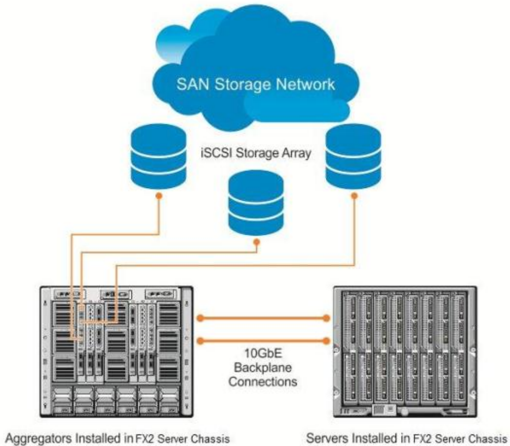
Figure 59. iSCSI Optimization Example
