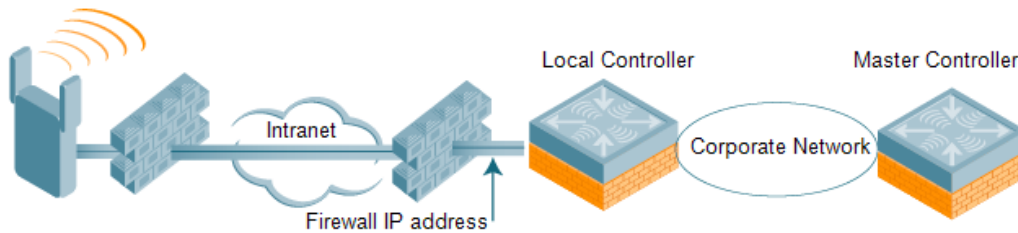
Figure 92 Remote AP in a Multi-Controller Environment
