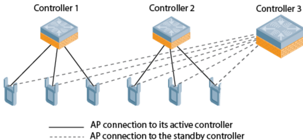
Figure 78 1:1 Active/Standby Deployment
