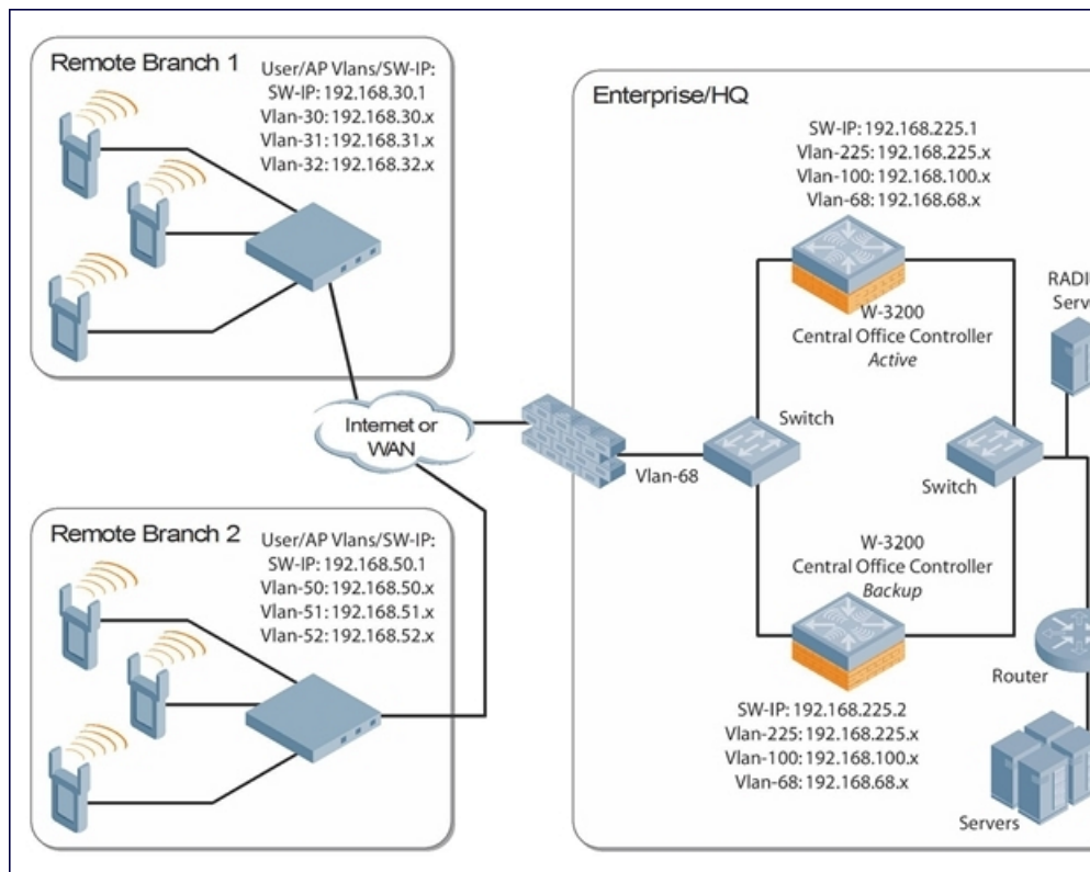
Figure 33 Sample OSPF Topology
