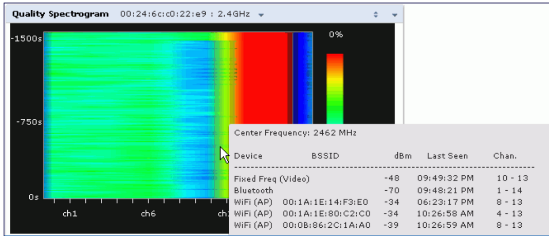
Figure 128 Quality Spectrogram
