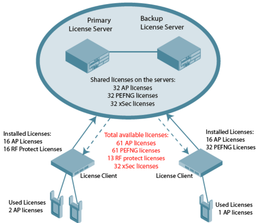
Figure 11 License Pool Reflecting Used licenses
