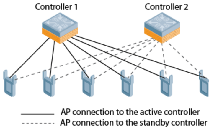
Figure 77 1:1 Active/Standby Deployment
