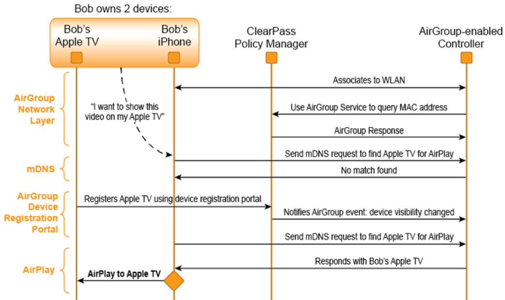
Figure 218 AirGroup Enables Personal Device Sharing
