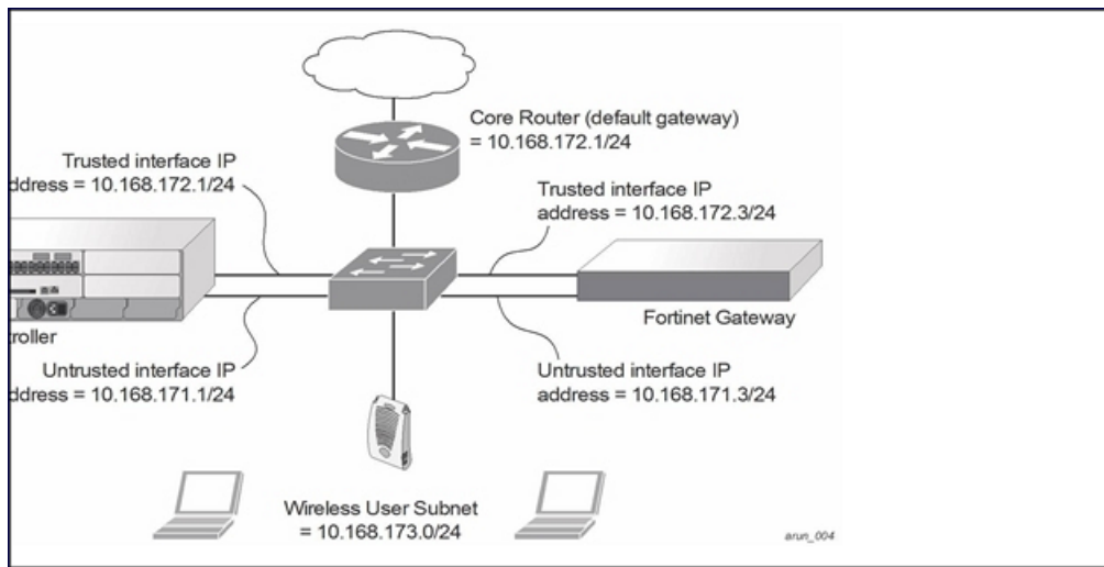
Figure 230 Example Route-Mode Topology
