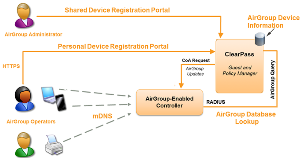
Figure 219 AirGroup in a Typical Wireless Deployment
