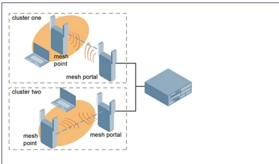
Figure 70 Sample Mesh Clusters
