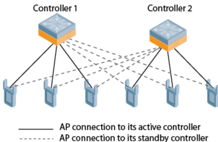
Figure 76 Active-Active HA Deployment
