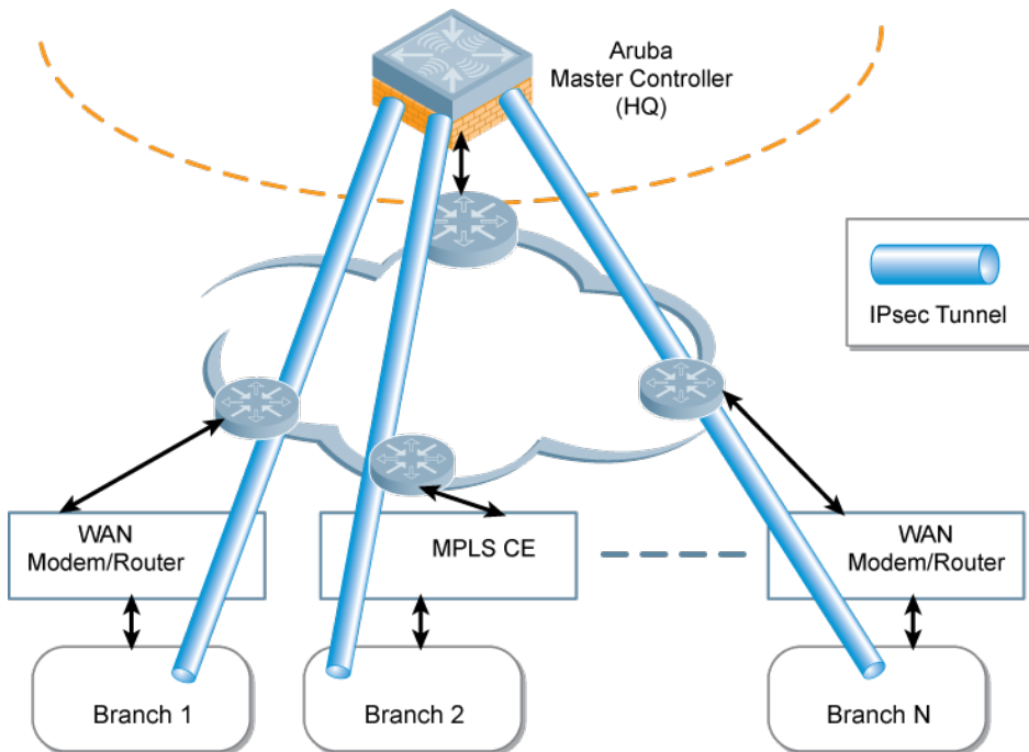
Figure 38 Branch Deployment Model with Master Controller in HQ
