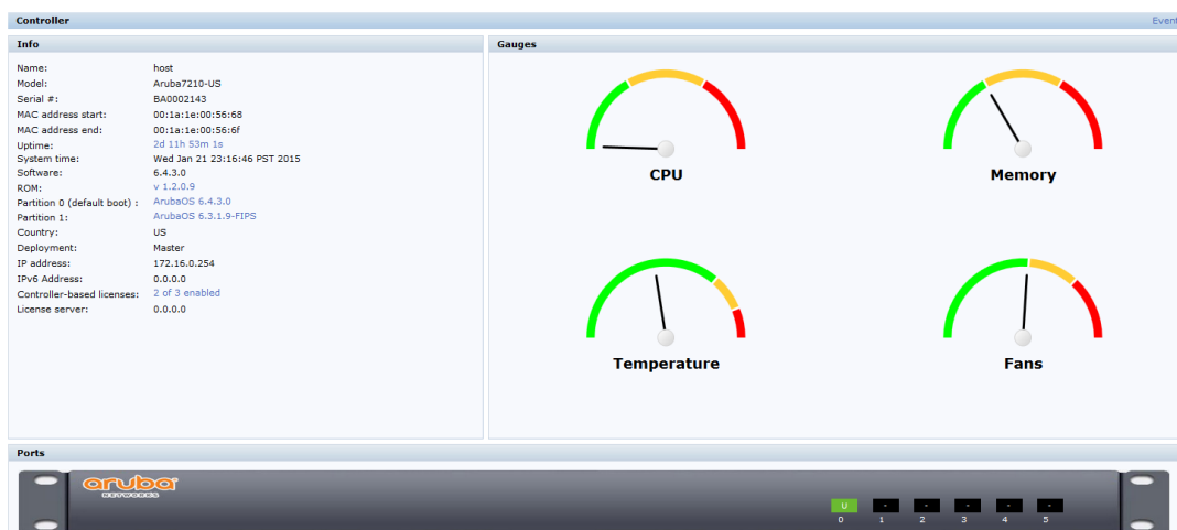
Figure 177 Controller Dashboard
