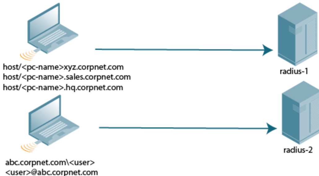
Figure 35 Server Group
