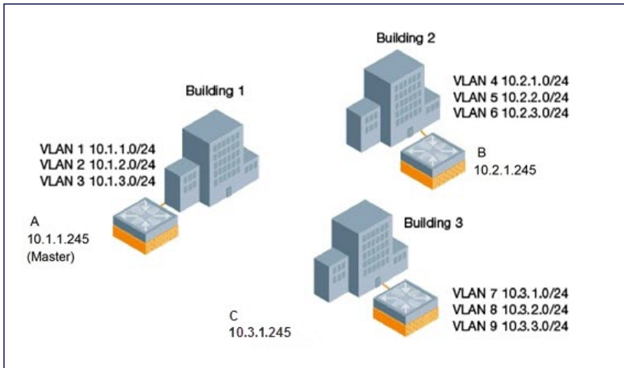
Figure 85 Example Configuration: Campus-Wide
