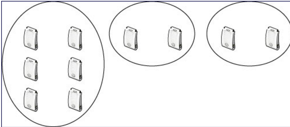
Figure 64 AP Groups
