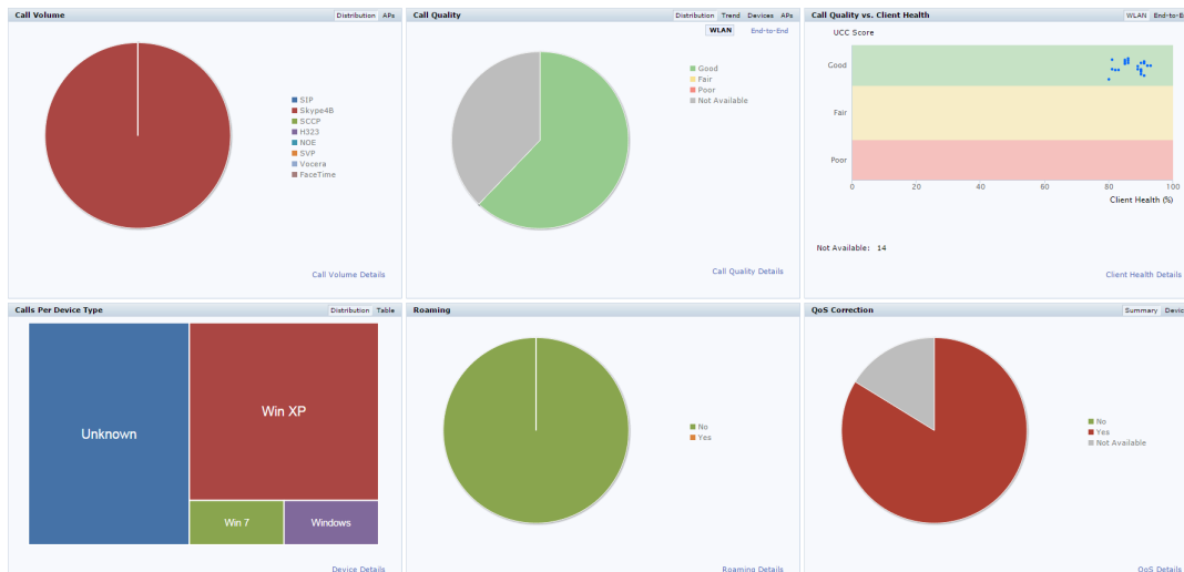
Figure 200 UCC Dashboard
