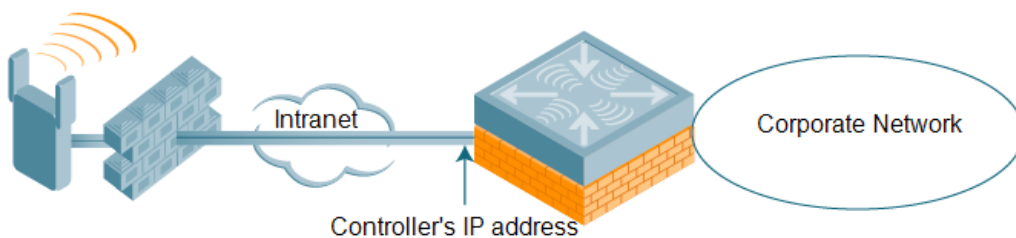
Figure 90 Remote AP with Controller on Public Network
