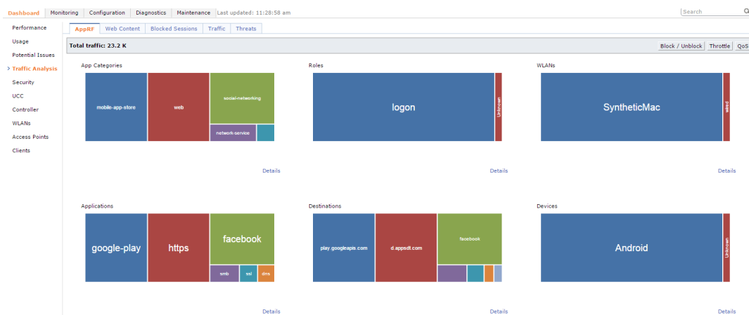
Figure 139 AppRF Page
