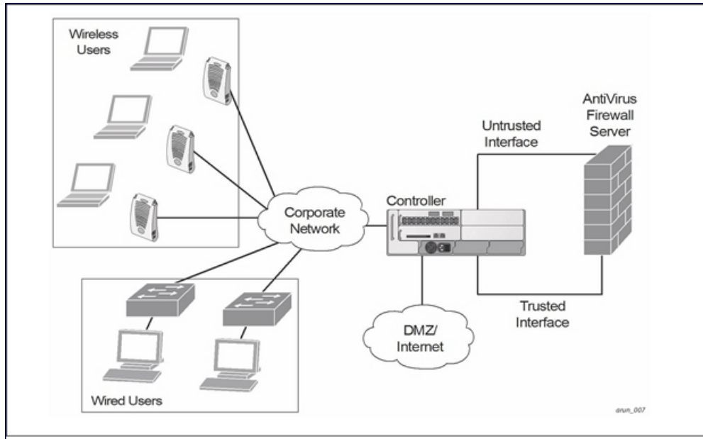
Figure 226 ESI-Fortinet Topology
