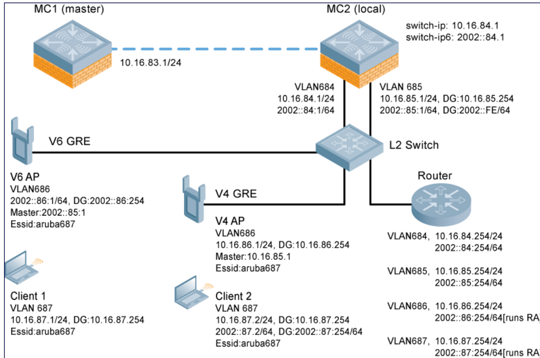
Figure 28 IPv6 Topology
