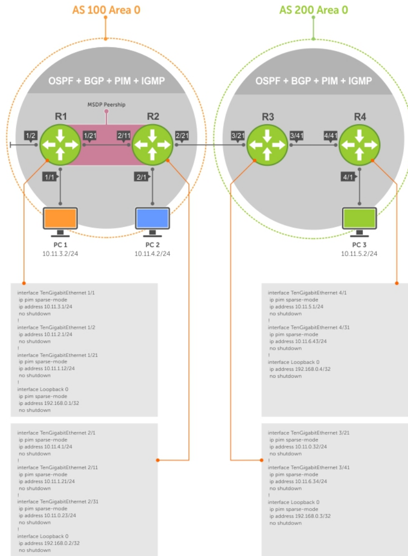
Figure 80. Configuring Interfaces for MSDP
