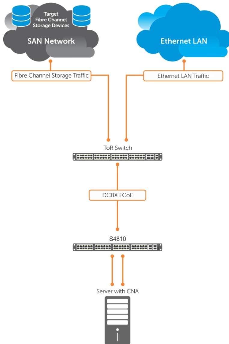
Figure 35. FIP Snooping on a Dell EMC Networking Switch
