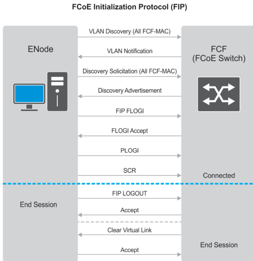
Figure 34. FIP Discovery and Login Between an ENode and an FCF
