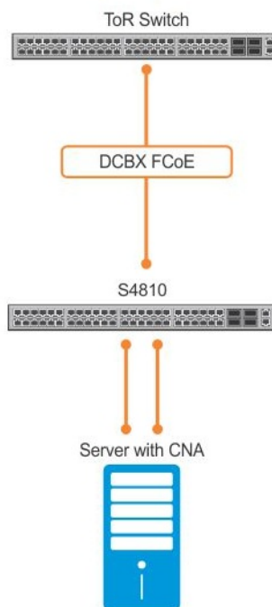
Figure 36. Configuration Example: FIP Snooping on a Switch
