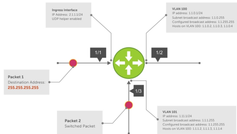
Figure 48. UDP Helper with Broadcast-All Addresses
