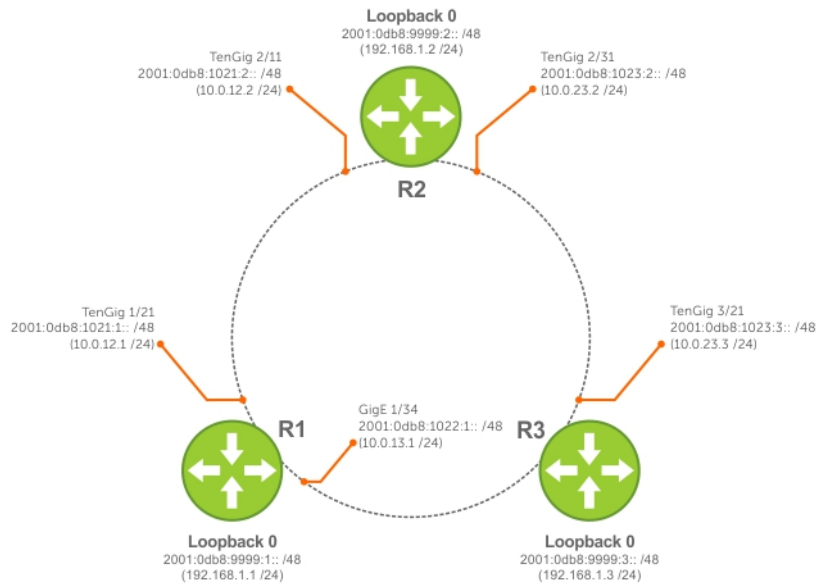
Figure 57. IPv6 IS-IS Sample Topology
