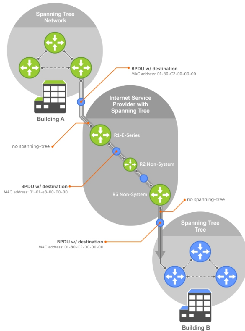
Figure 116. VLAN Stacking with L2PT
