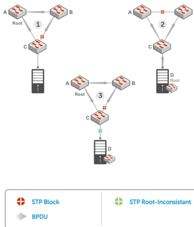
Figure 120. STP Root Guard Prevents Bridging Loops
