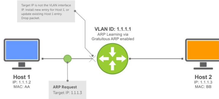
Figure 47. ARP Learning via ARP Request with ARP Learning via Gratuitous ARP Enabled
