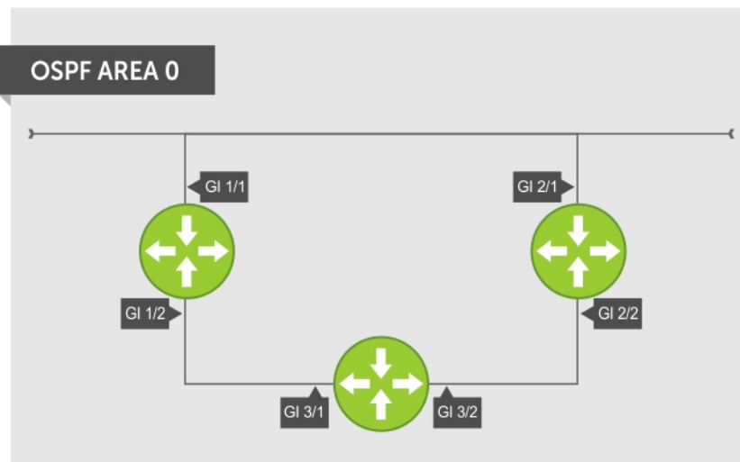
Figure 96. Basic Topology and CLI Commands for OSPFv2
