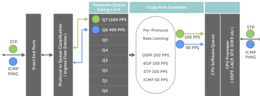
Figure 26. CoPP Implemented Versus CoPP Not Implemented
