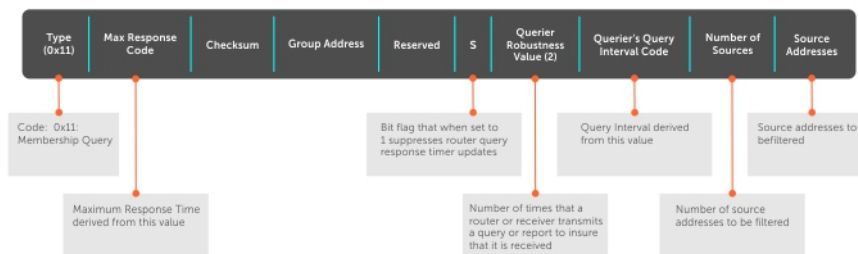
Figure 42. IGMP Version 3 Packet Structure
