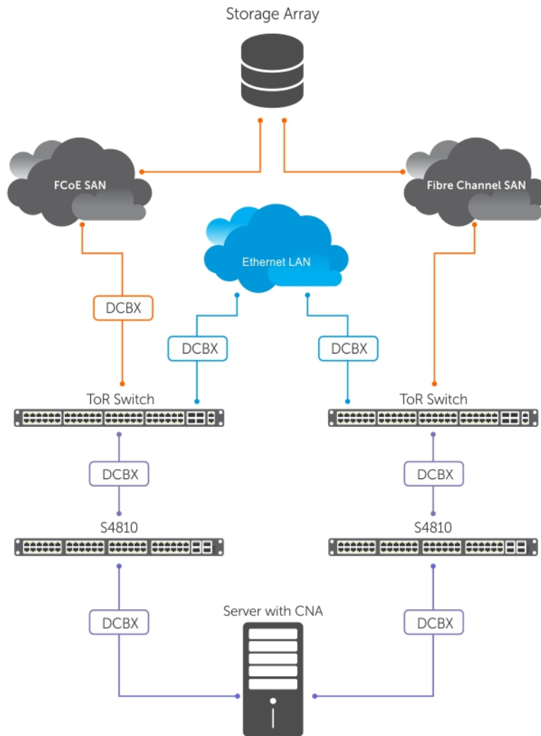
Figure 31. PFC and ETS Applied to LAN, IPC, and SAN Priority Traffic
