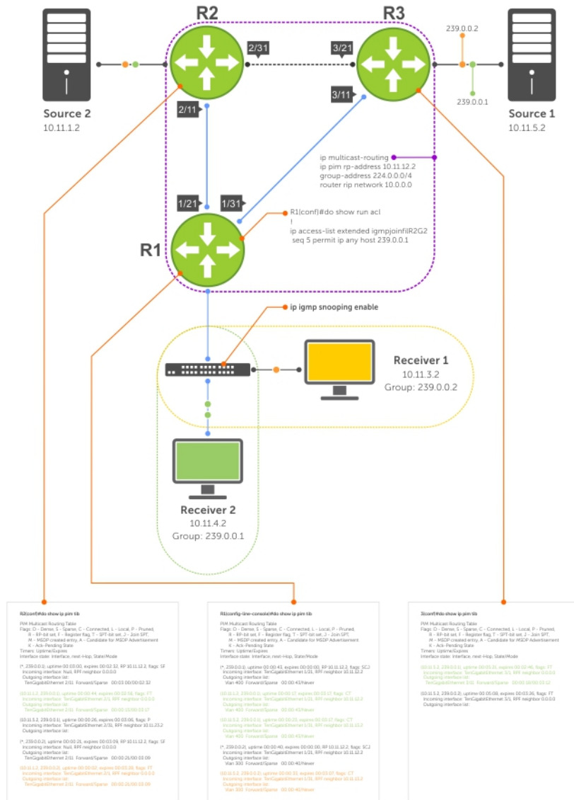
Figure 91. Preventing a Source from Transmitting to a Group
