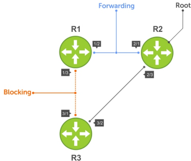
Figure 89. MSTP with Three VLANs Mapped to Two Spanning Tree Instances
