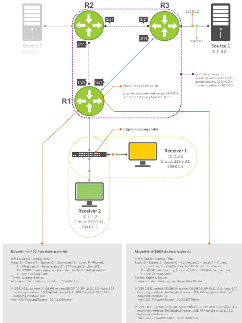
Figure 90. Preventing a Host from Joining a Group
