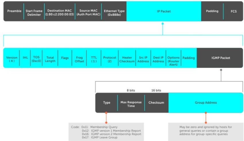
Figure 41. IGMP Messages in IP Packets
