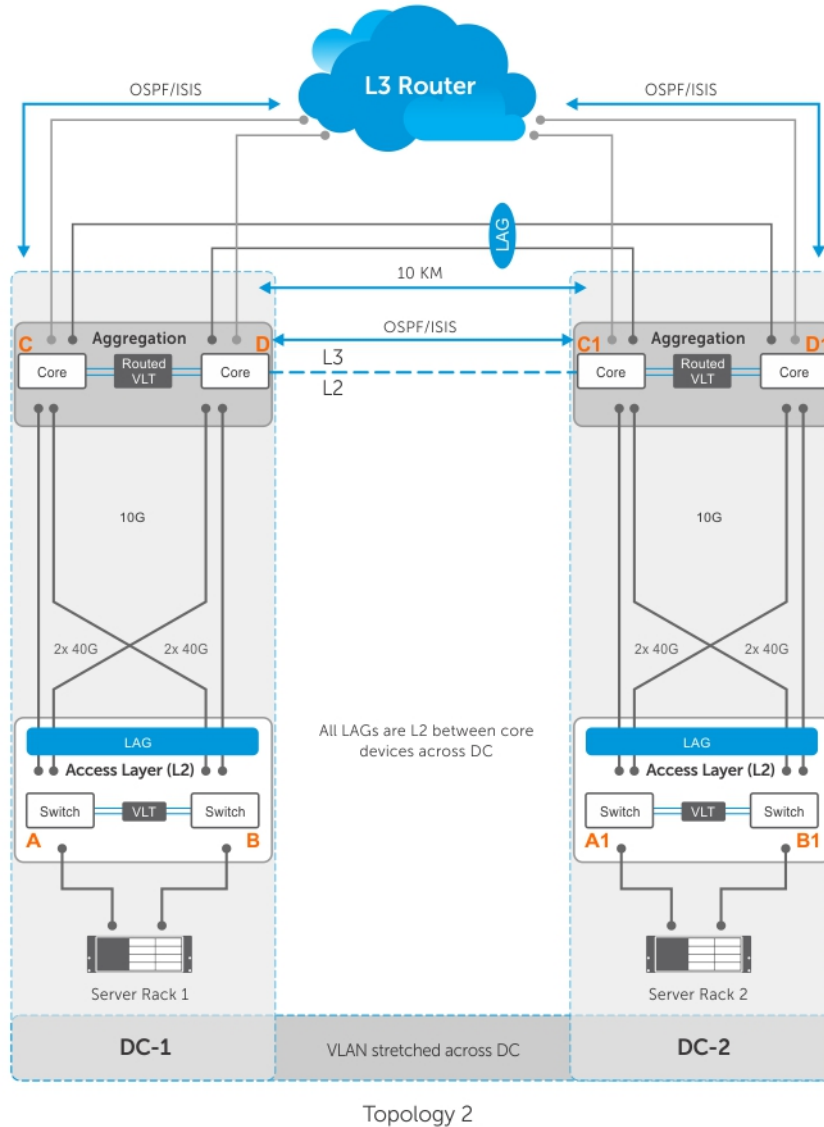
Figure 141. Sample Configuration for a VLT Proxy Gateway
