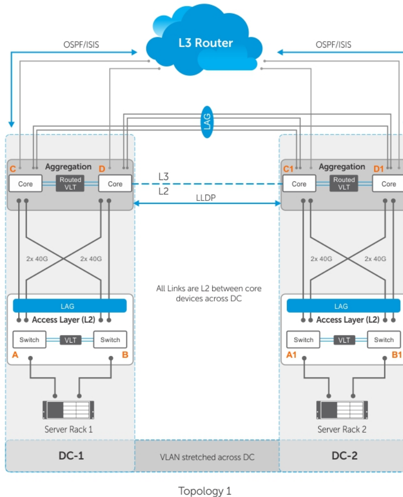
Figure 140. Sample Configuration for a VLT Proxy Gateway
