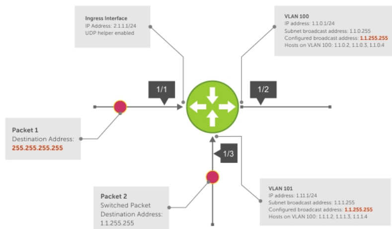
Figure 50. UDP Helper with Configured Broadcast Addresses
