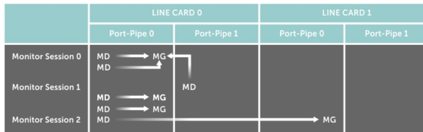
Figure 97. Port Monitoring Configurations
