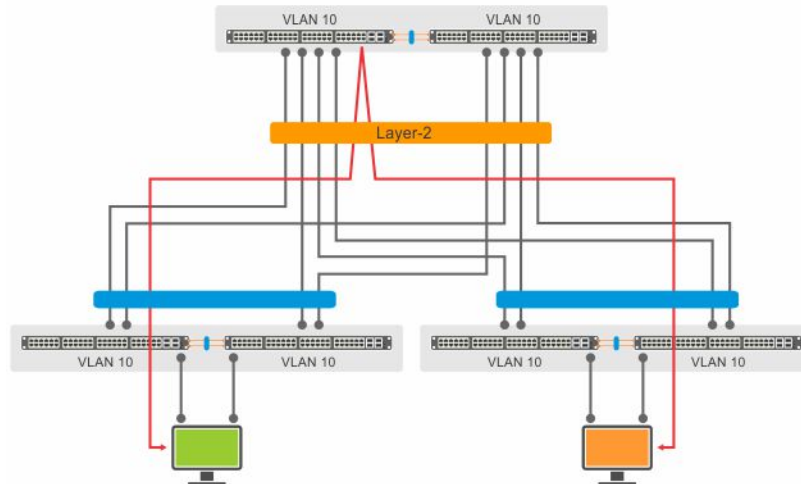
Figure 130. Layer-2 Traffic in VLT Domains
