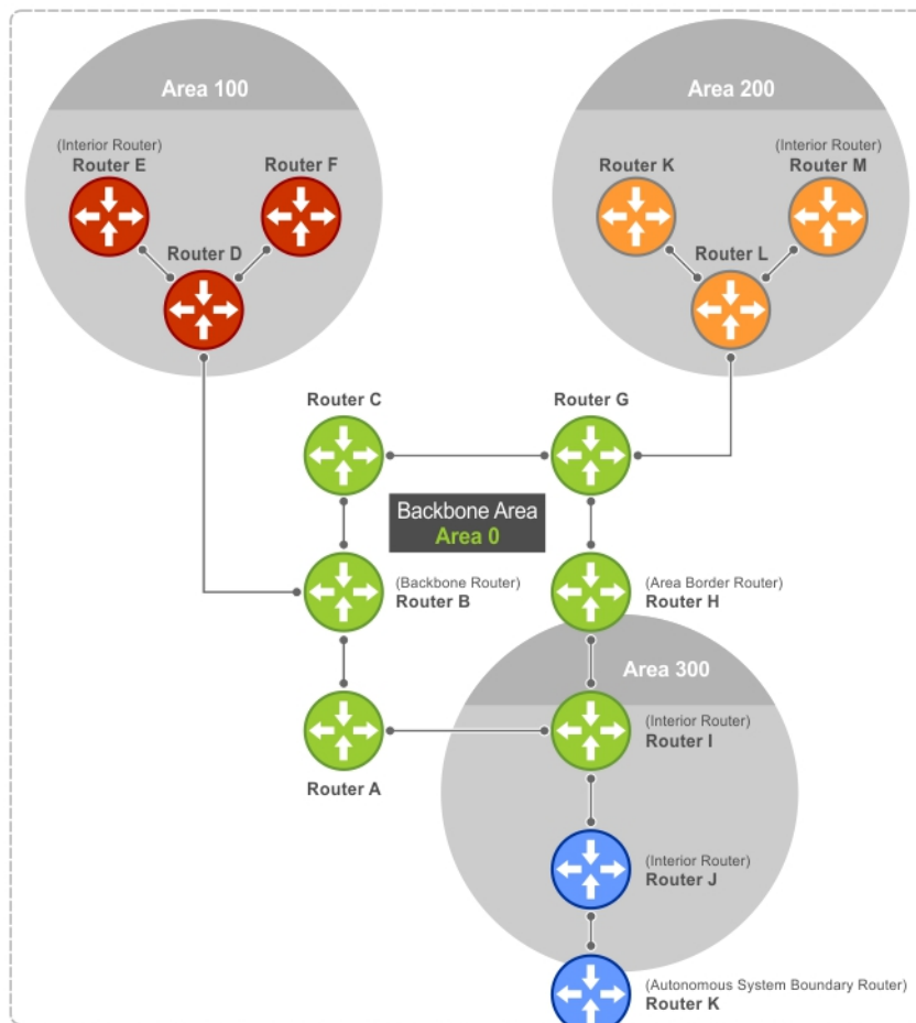
Figure 93. Autonomous System Areas
