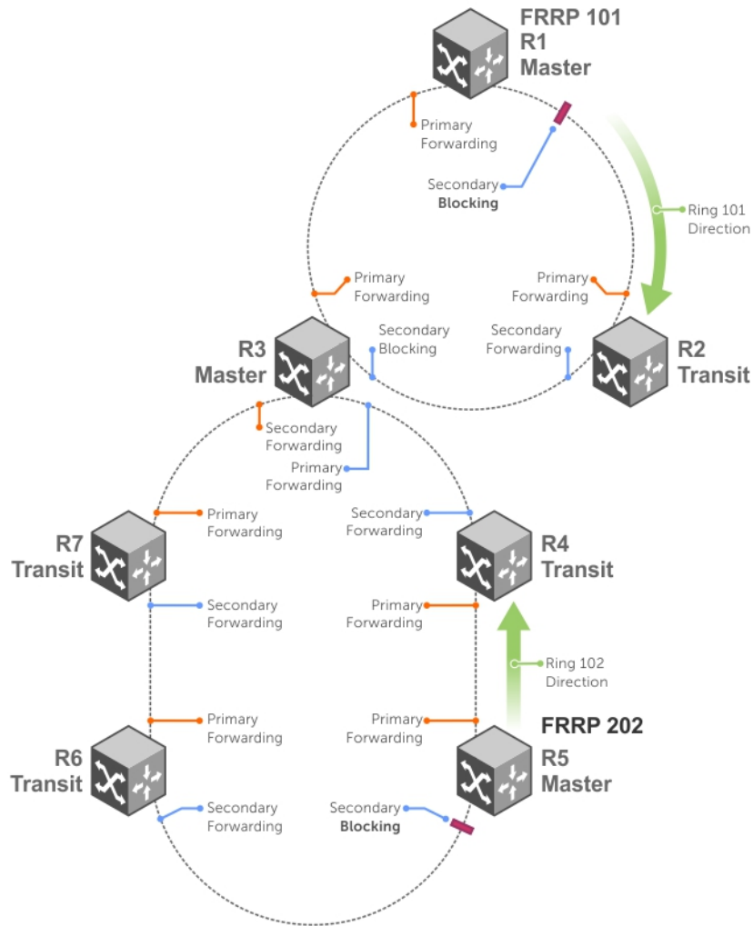
Figure 37. Example of Multiple Rings Connected by Single Switch
