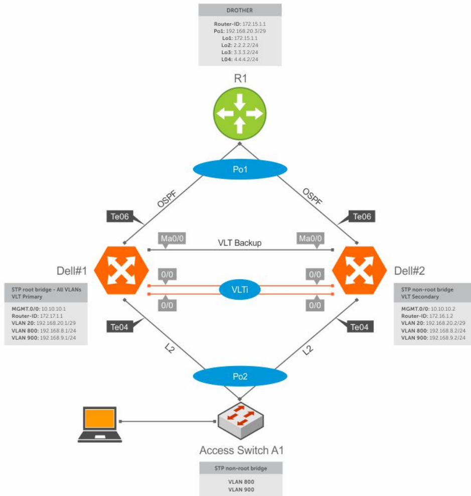
Figure 136. Peer Routing Configuration Example
