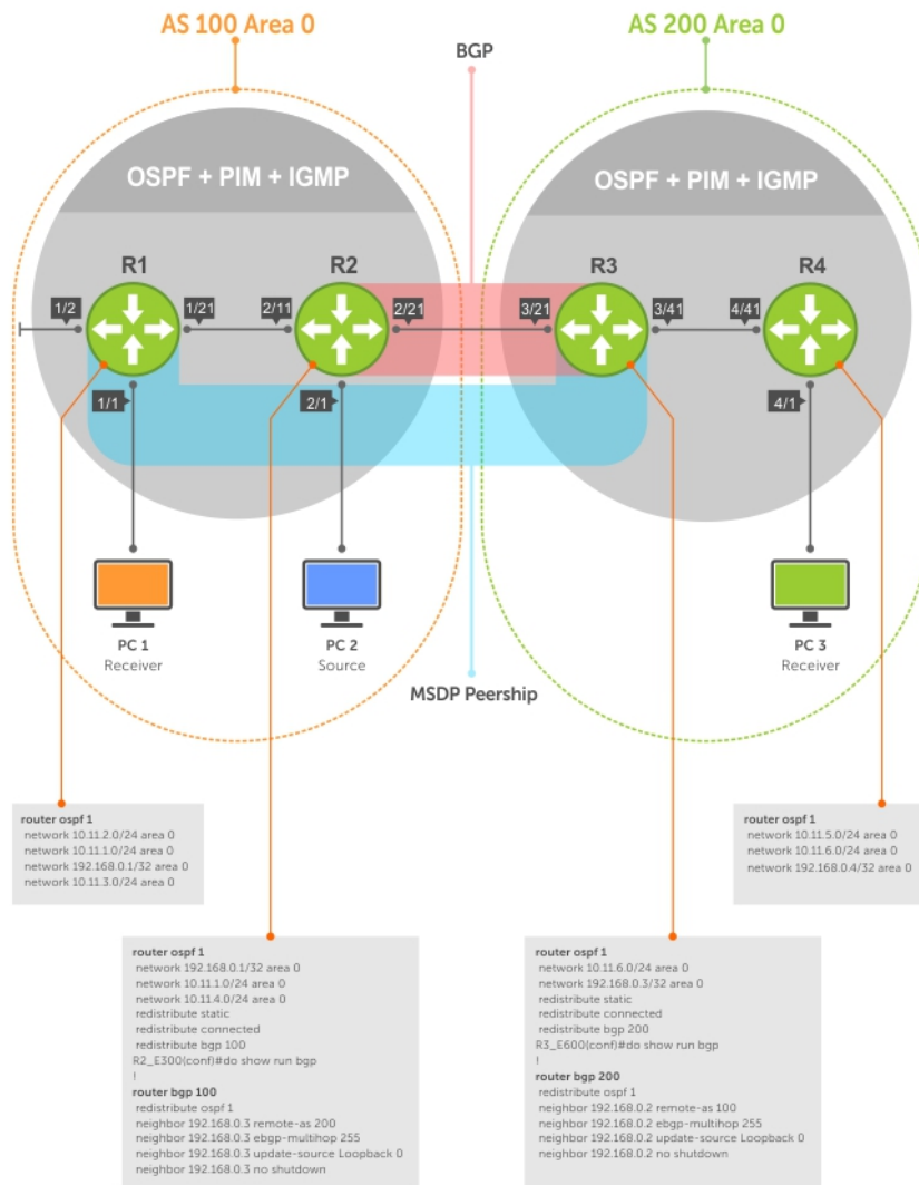
Figure 81. Configuring OSPF and BGP for MSDP
