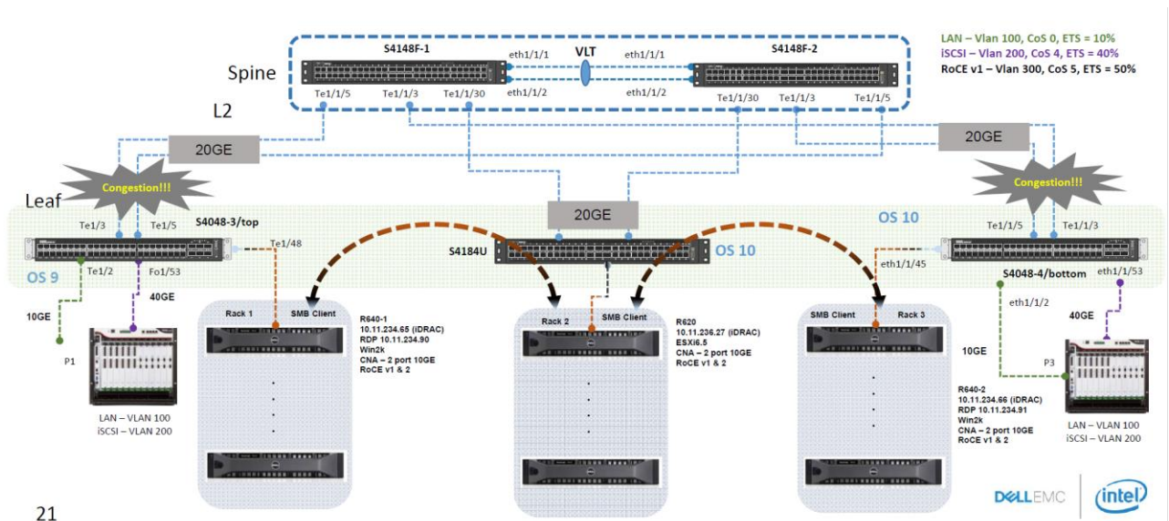
Figure 1 Dell EMC Networking RoCE v1 Reference Environment.
