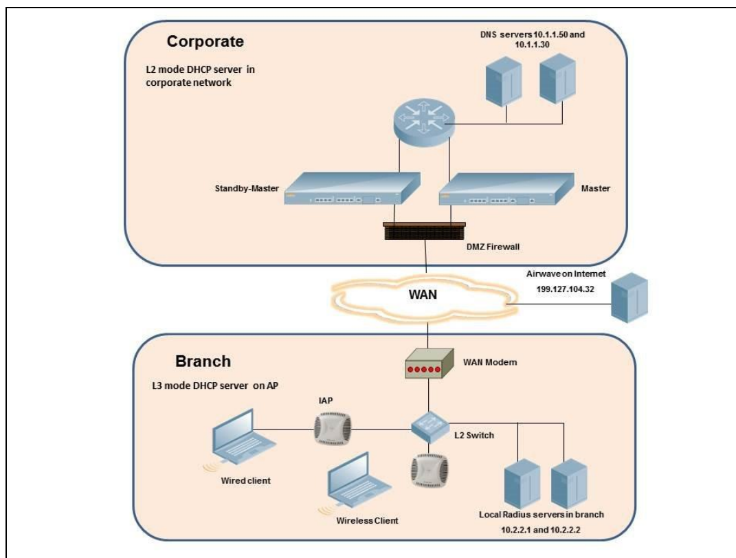
Figure 121 Scenario 2—IPsec: Single Datacenter with Multiple controllers for Redundancy
