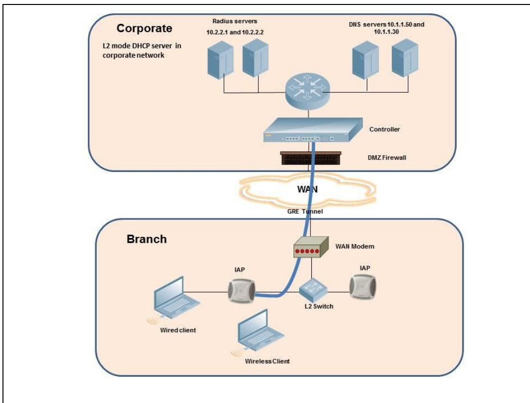
Figure 124 Scenario 4 - GRE: Single Datacenter Deployment with No Redundancy
