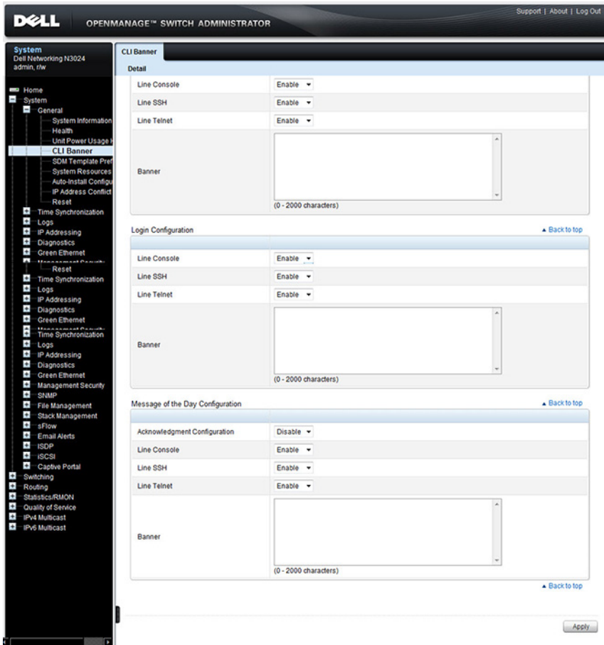
Figure 12-5. CLI Banner
