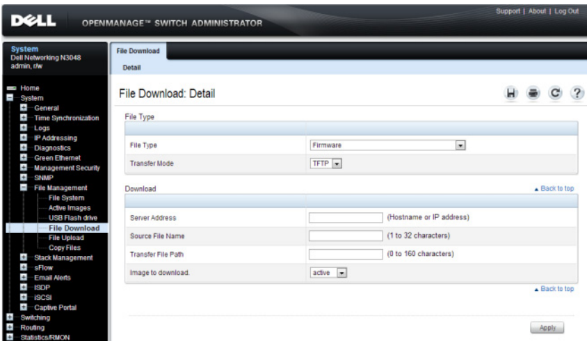
Figure 14-4. File Download
