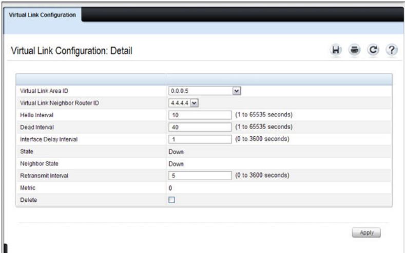
Figure 35-30. OSPFv3 Virtual Link Configuration
