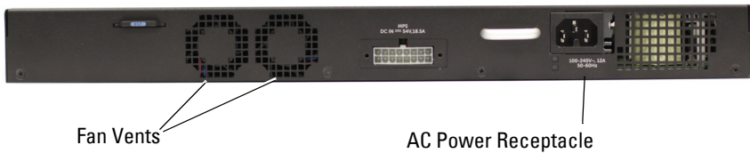
Figure 3-3. Dell Networking N1500 Series Back Panel
