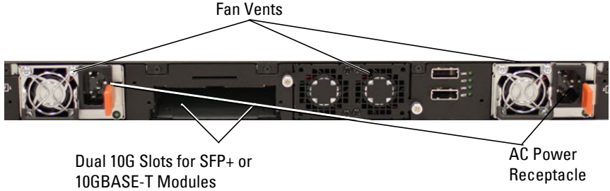
Figure 3-20. Dell EMC Networking N3000/N3000E-ON Series Back Panel
