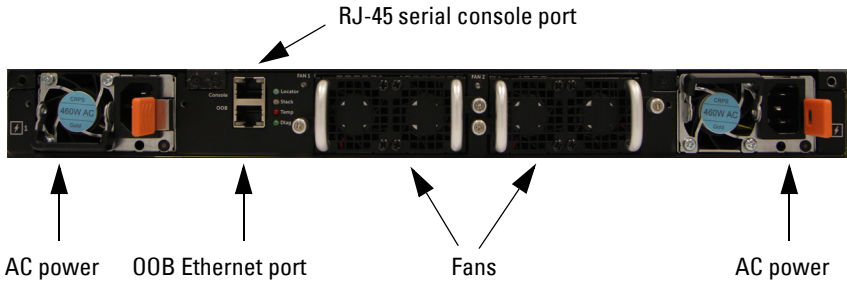
Figure 3-22. Dell Networking N4000 Series Back Panel
