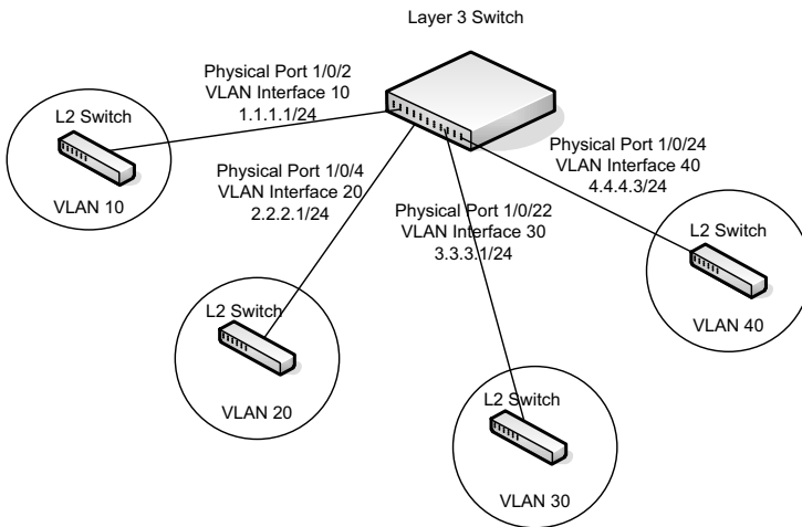
Figure 20-14. Policy-Based Routing on VLAN Interfaces Example
