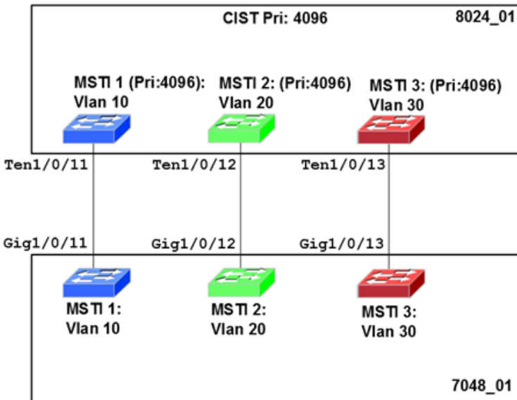
Figure 22-4. MSTP with Multiple Forwarding Paths
