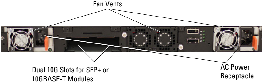
Figure 3-14. Dell Networking N3000 Series Back Panel
