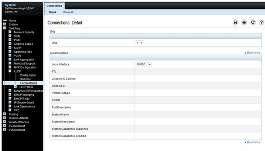
Figure 23-9. LLDP Connections
