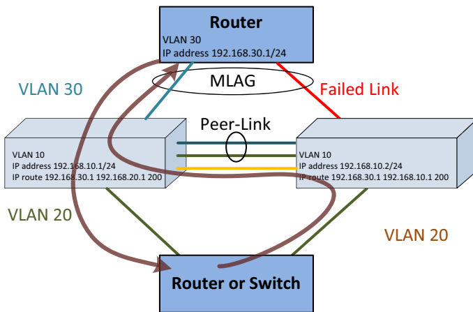
Figure 26-16. Degenerate Routing Topology
