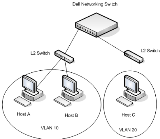
Figure 30-1. Inter-VLAN Routing
