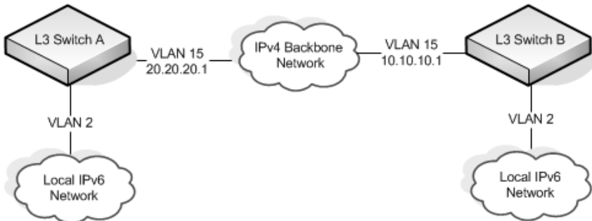
Figure 32-38. IPv4 and IPv6 Interconnection Example
