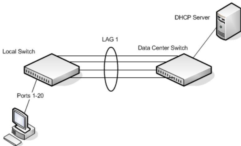
Figure 25-25. DHCP Snooping Configuration Topology
