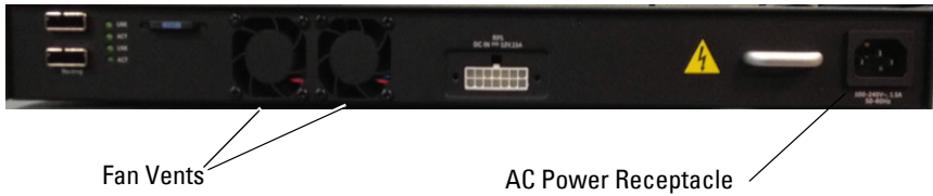
Figure 3-7. Dell Networking N2000 Series Back Panel
