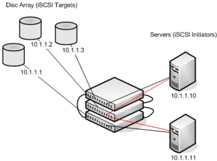
Figure 9-15. NSF and a Storage Area Network
