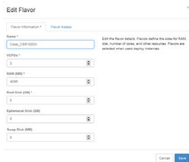
Figure 17-3. Cisco_CSR1000v Flavor
