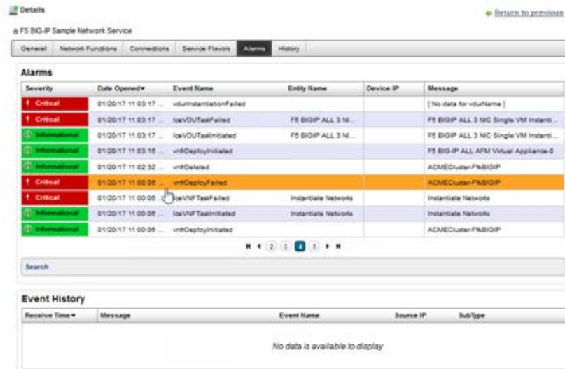
Figure 18-17. Network Service Alarms Details
