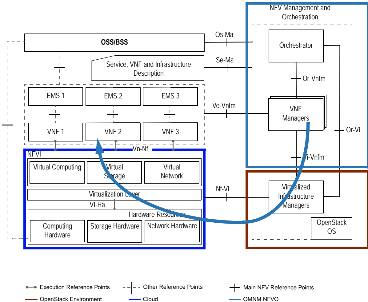
Figure 17-1. OMNM and OpenStack Interaction
