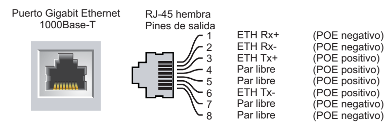
Figura 5 Pines del puerto Gigabit Ethernet
