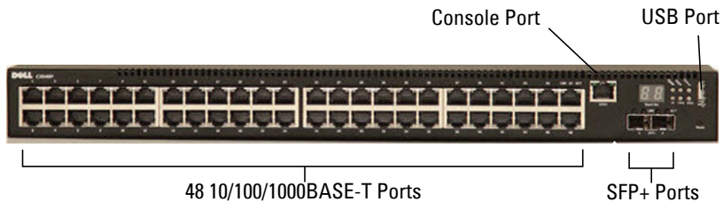
Figure 3-9. Dell EMC Networking N2048 Switch with 48 10/100/1000BASE-T Ports (Front Panel)
