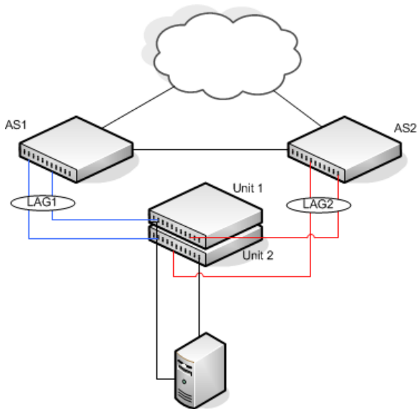
Figure 8-12. Data Center Stack Topology
