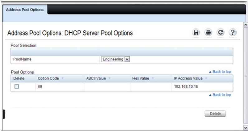
Figure 30-10. View Address Pool Options
