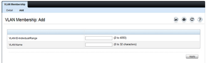
Figure 20-5. Add VLAN
