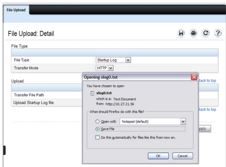
Figure 13-7. File Upload
