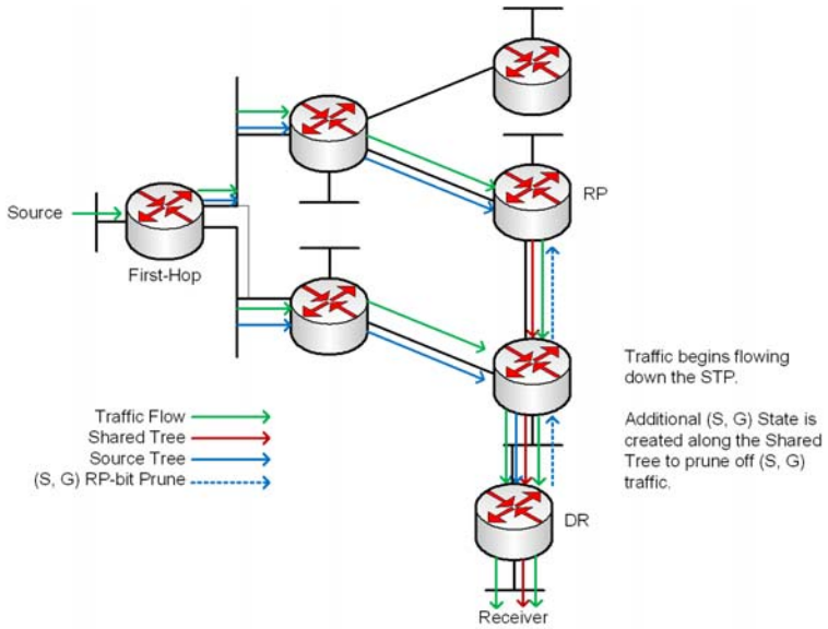
Figure 46-5. PIM-SM SPT—Part 2
