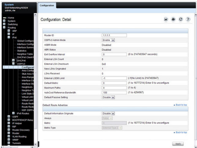
Figure 34-18. OSPFv3 Configuration
