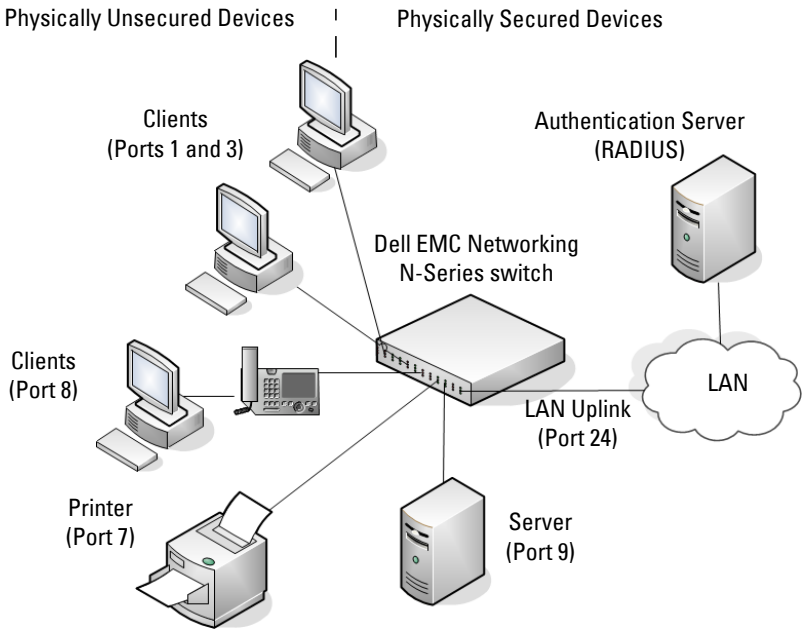
Figure 9-12. 802.1X Example
