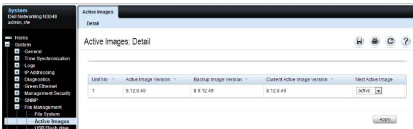
Figure 13-2. Active Images
