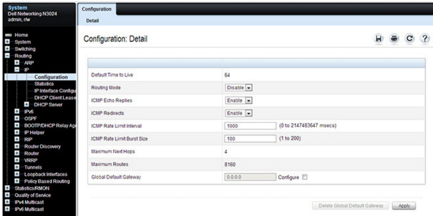
Figure 31-1. IP Configuration
