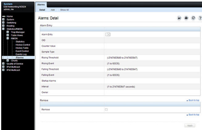
Figure 15-20. RMON Alarms
