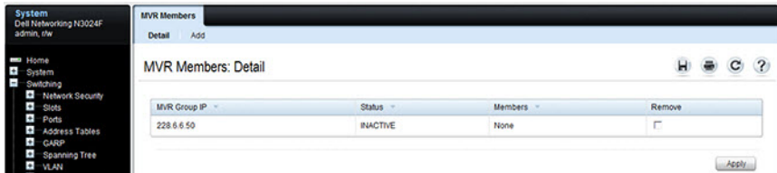
Figure 24-24. MVR Members
