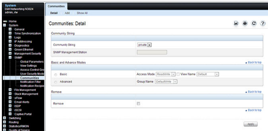
Figure 12-9. SNMP Communities
