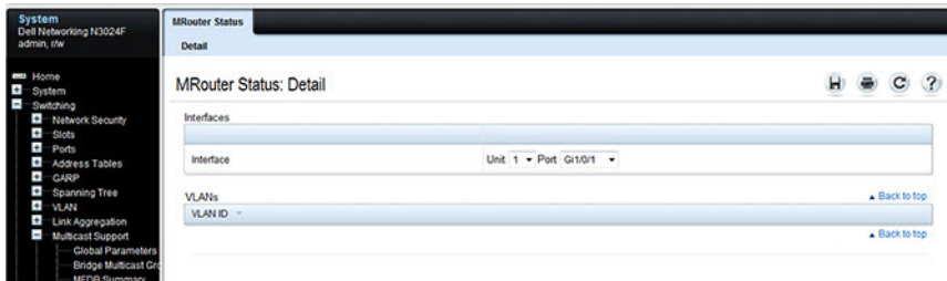
Figure 24-5. MRouter Status
