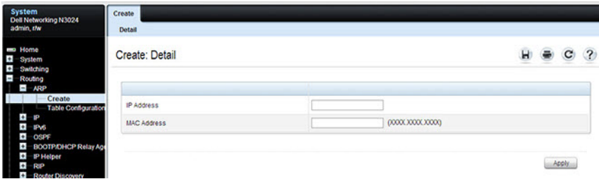
Figure 31-3. ARP Create
