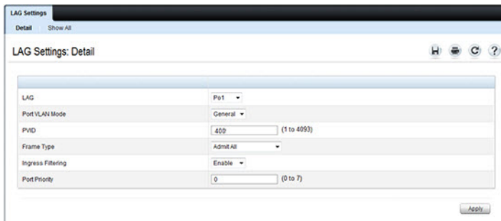
Figure 20-30. LAG Settings
