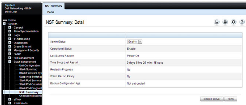
Figure 8-9. NSF Summary
