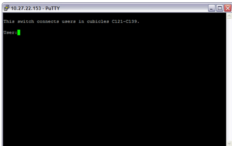
Figure 11-25. Verify MOTD
