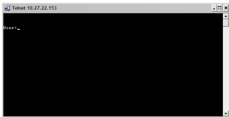
Figure 11-4. Telnet Session
