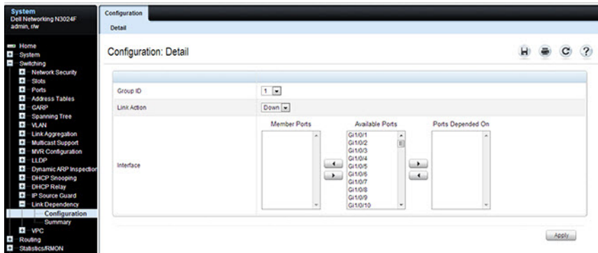
Figure 17-4. Link Dependency Configuration
