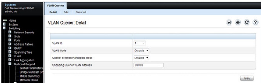
Figure 24-10. VLAN Querier
