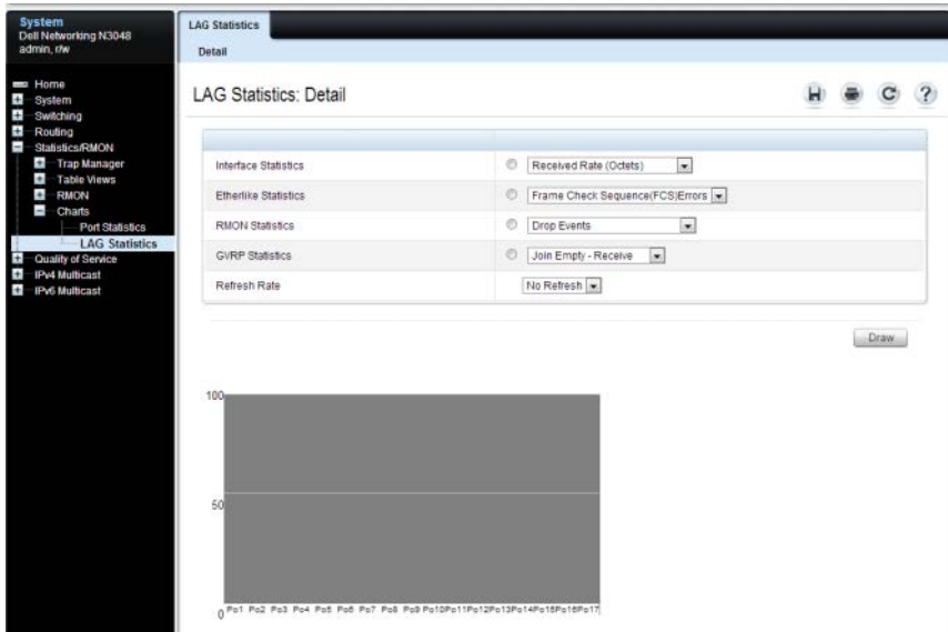
Figure 15-23. LAG Statistics
