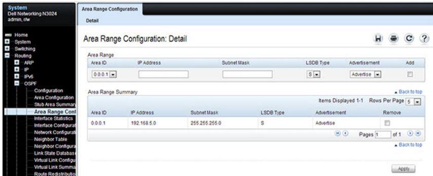
Figure 34-6. OSPF Area Range Configuration
