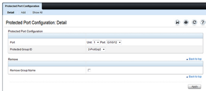
Figure 23-6. Add Protected Ports
