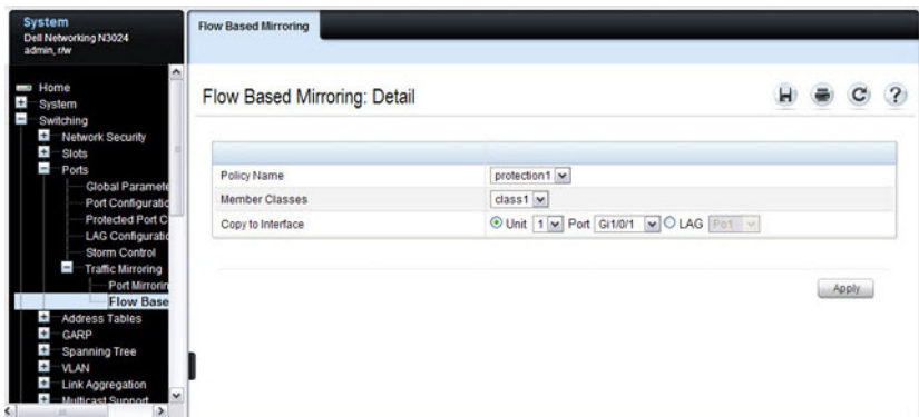
Figure 43-16. Flow-Based Mirroring
