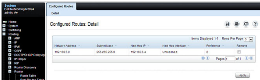
Figure 31-11. Configured Routes
