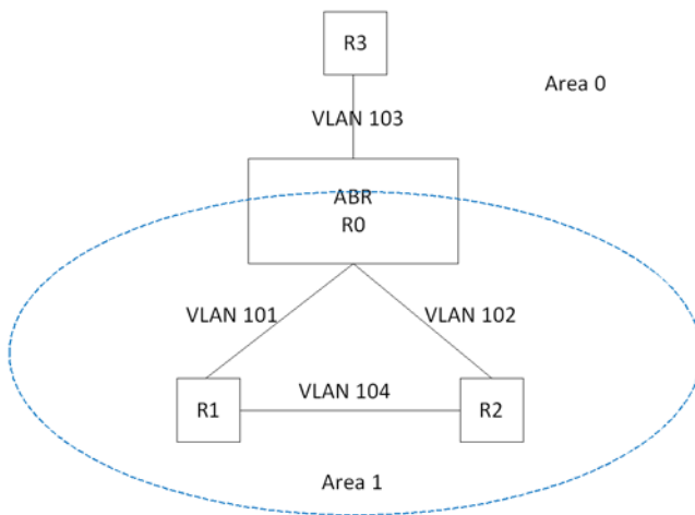
Figure 34-39. Static Area Range Cost Example Topology
