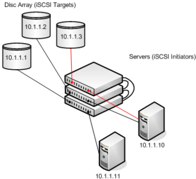
Figure 16-2. iSCSI Optimization
