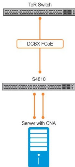
Figure 43. Configuration Example: FIP Snooping on a Switch
