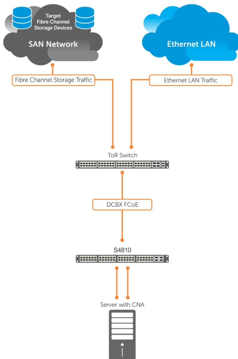
Figure 42. FIP Snooping on a Dell EMC Networking Switch
