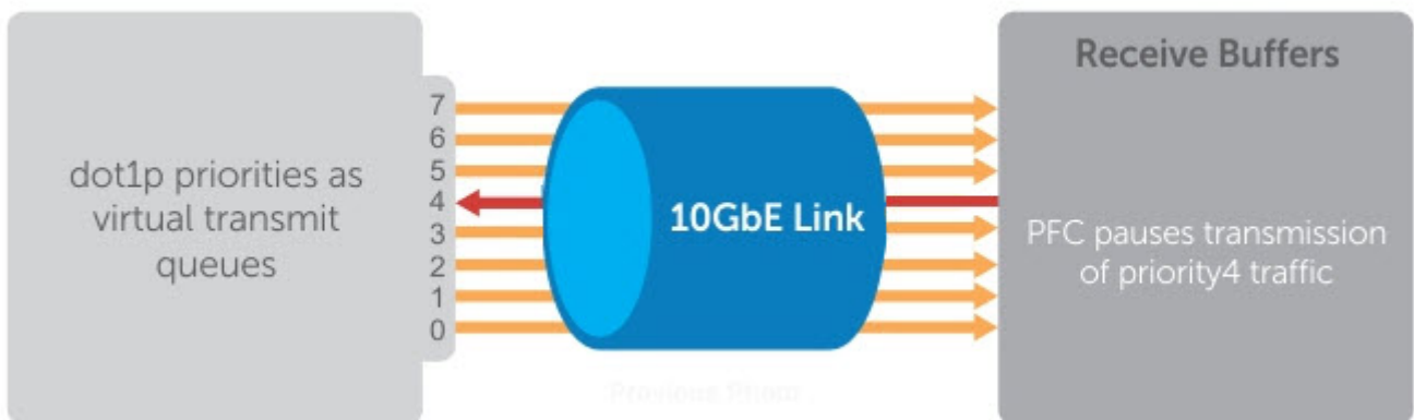
Figure 32. Illustration of Traffic Congestion
