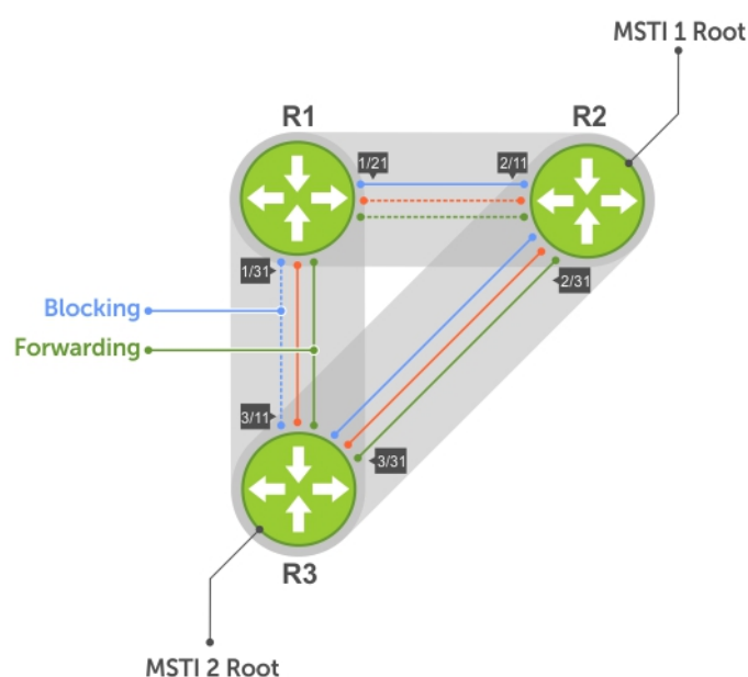
Figure 97. MSTP with Three VLANs Mapped to TWO Spanning Tree Instances
