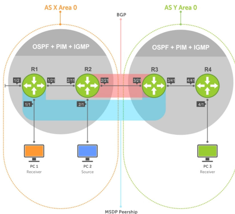
Figure 87. Multicast Source Discovery Protocol (MSDP)
