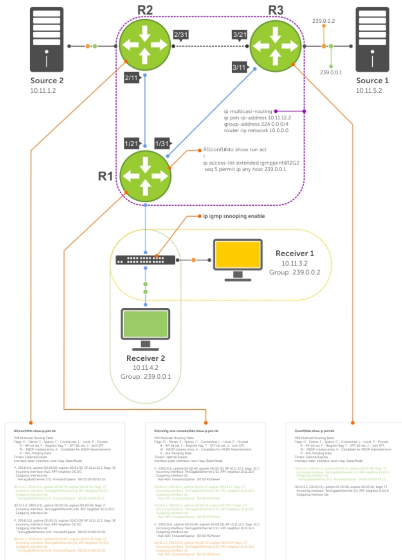
Figure 100. Preventing a Source from Transmitting to a Group
