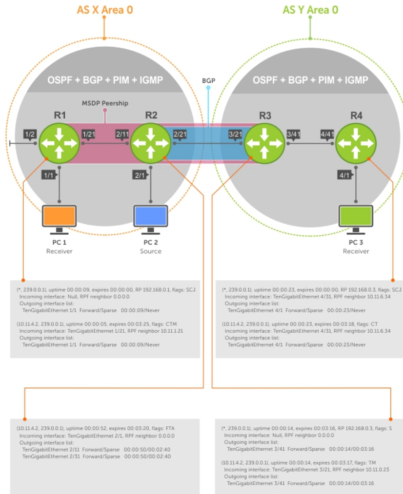
Figure 96. MSDP with Anycast RP
