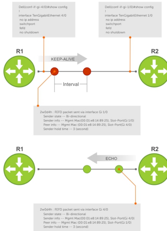
Figure 78. Configuring Far-End Failure Detection
