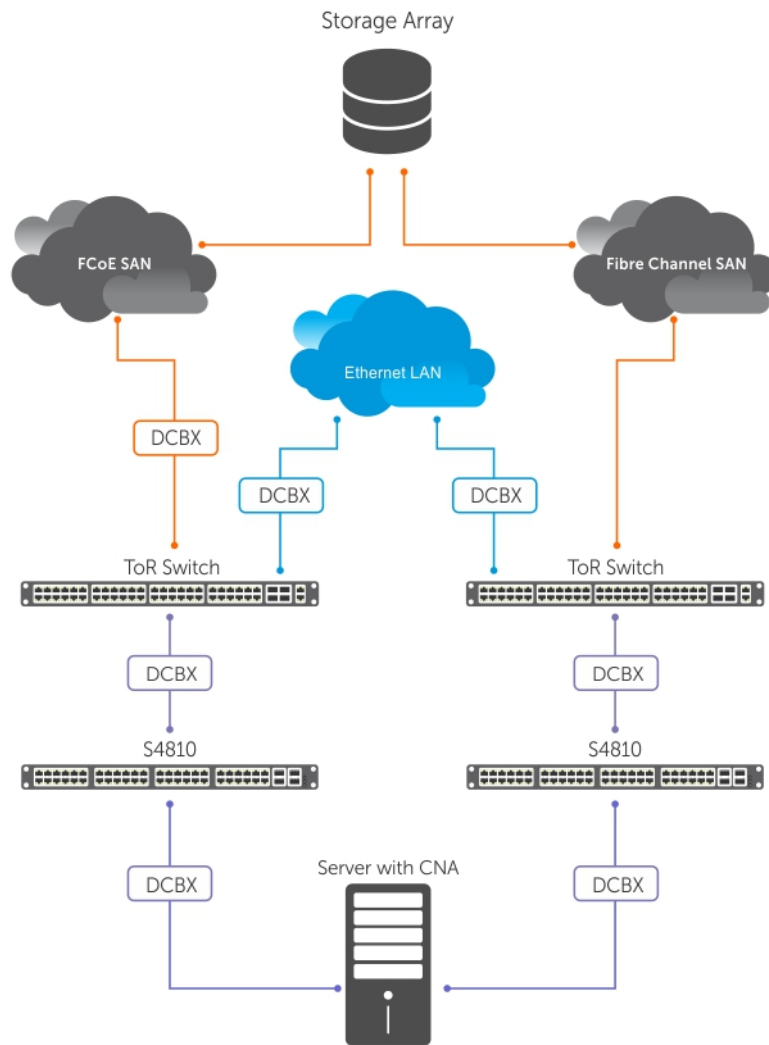
Figure 35. PFC and ETS Applied to LAN, IPC, and SAN Priority Traffic
