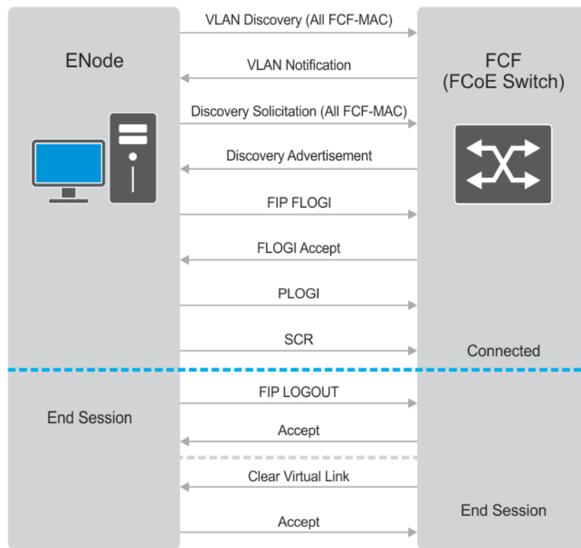
Figure 41. FIP Discovery and Login Between an ENode and an FCF
