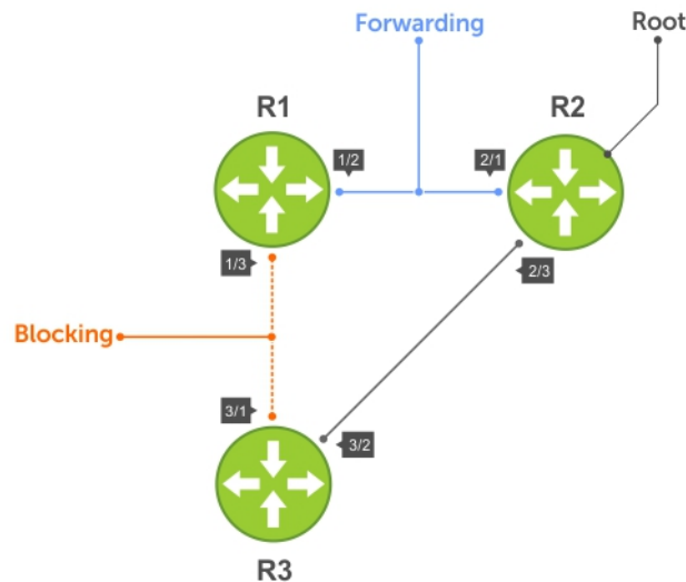
Figure 98. MSTP with Three VLANs Mapped to Two Spanning Tree Instances
