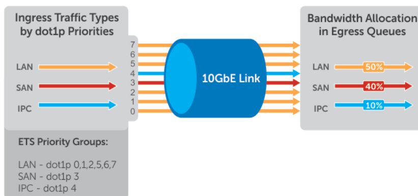
Figure 33. Enhanced Transmission Selection
