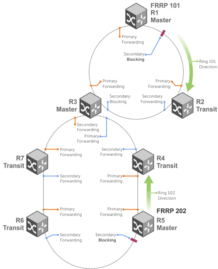
Figure 44. Example of Multiple Rings Connected by Single Switch
