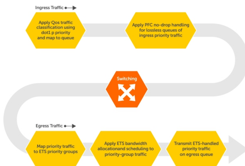
Figure 34. DCB PFC and ETS Traffic Handling
