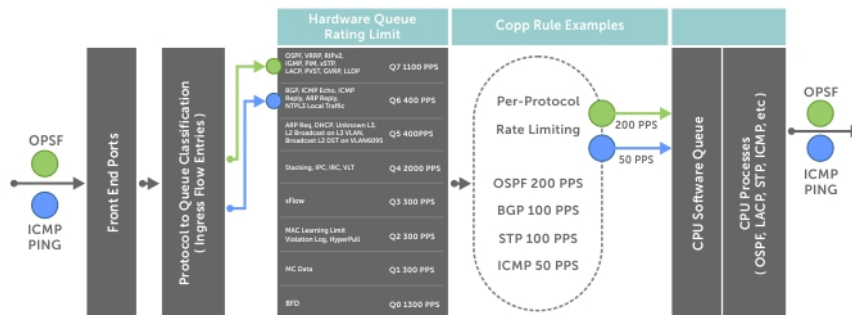
Figure 30. Control Plane Policing
