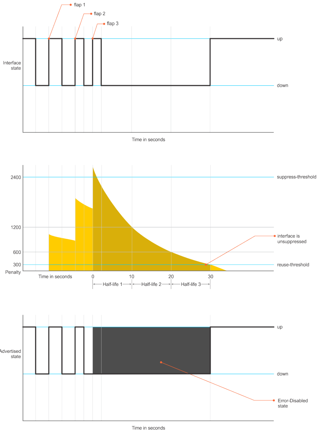
Figure 53. Interface State Change
