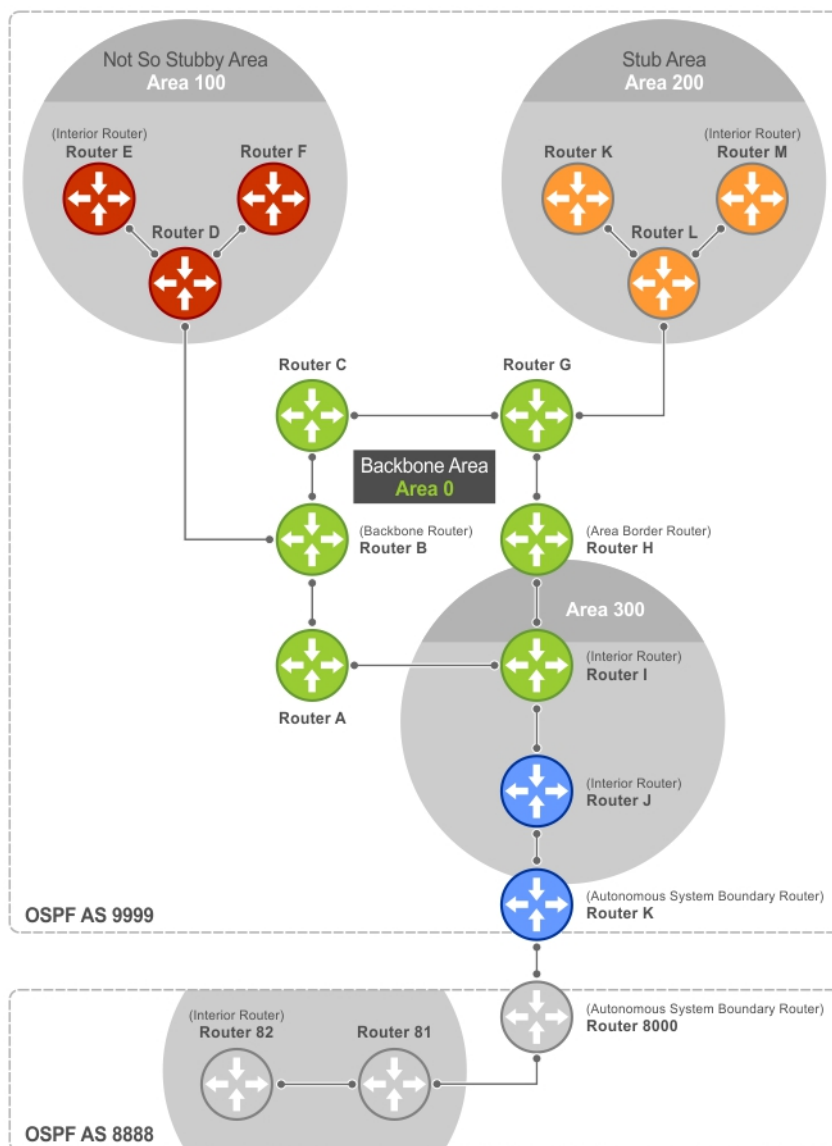
Figure 103. OSPF Routing Examples
