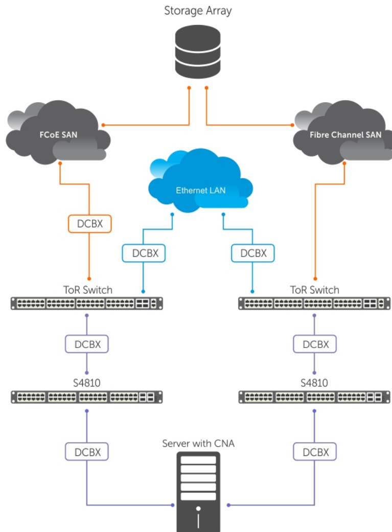
Figure 36. PFC and ETS Applied to LAN, IPC, and SAN Priority Traffic
