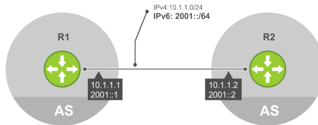
Figure 29. Configure IPv6 NH to advertise IPv6 prefix over IPv4 neighbor
