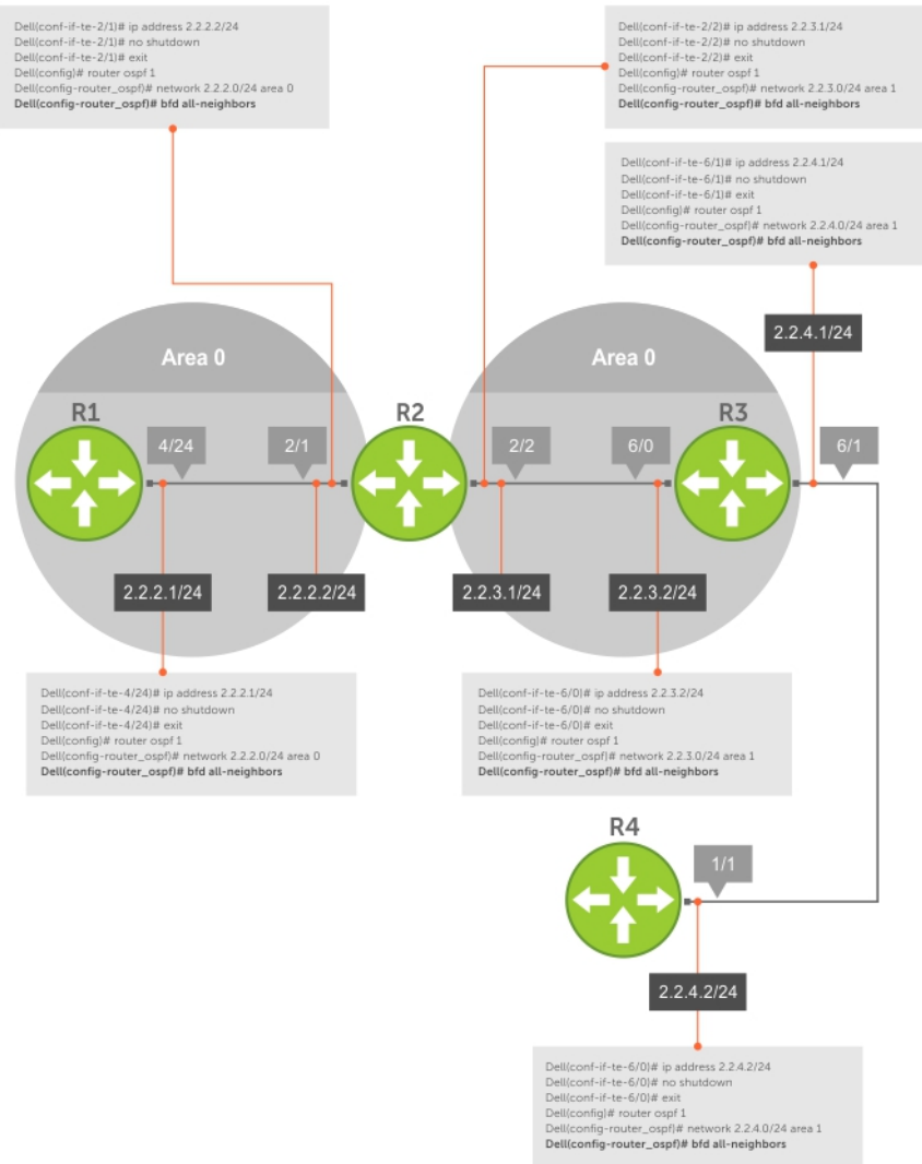
Figure 16. Establishing Sessions with OSPF Neighbors
