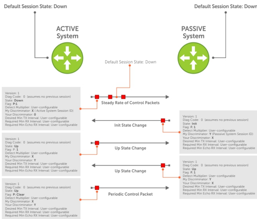
Figure 12. BFD Three-Way Handshake State Changes
