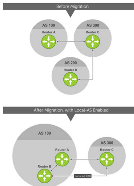
Figure 25. Before and After AS Number Migration with Local-AS Enabled
