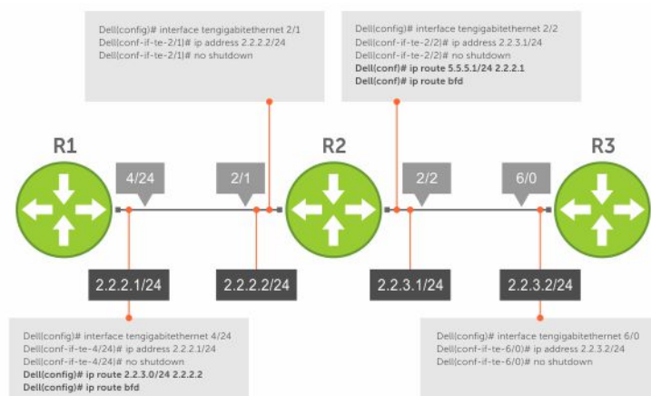
Figure 15. Establishing Sessions for Static Routes
