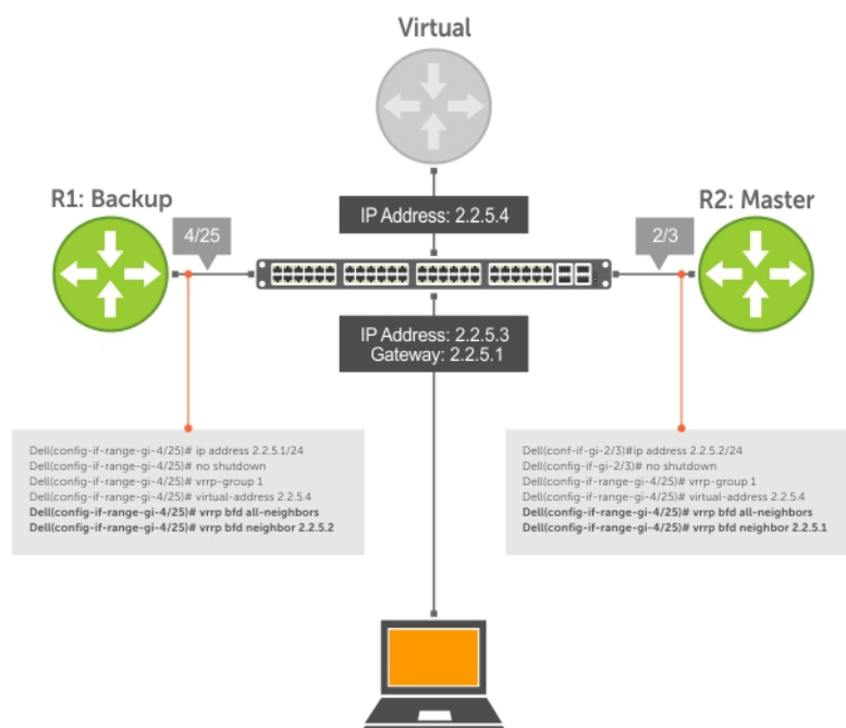
Figure 19. Establishing Sessions with All VRRP Neighbors
