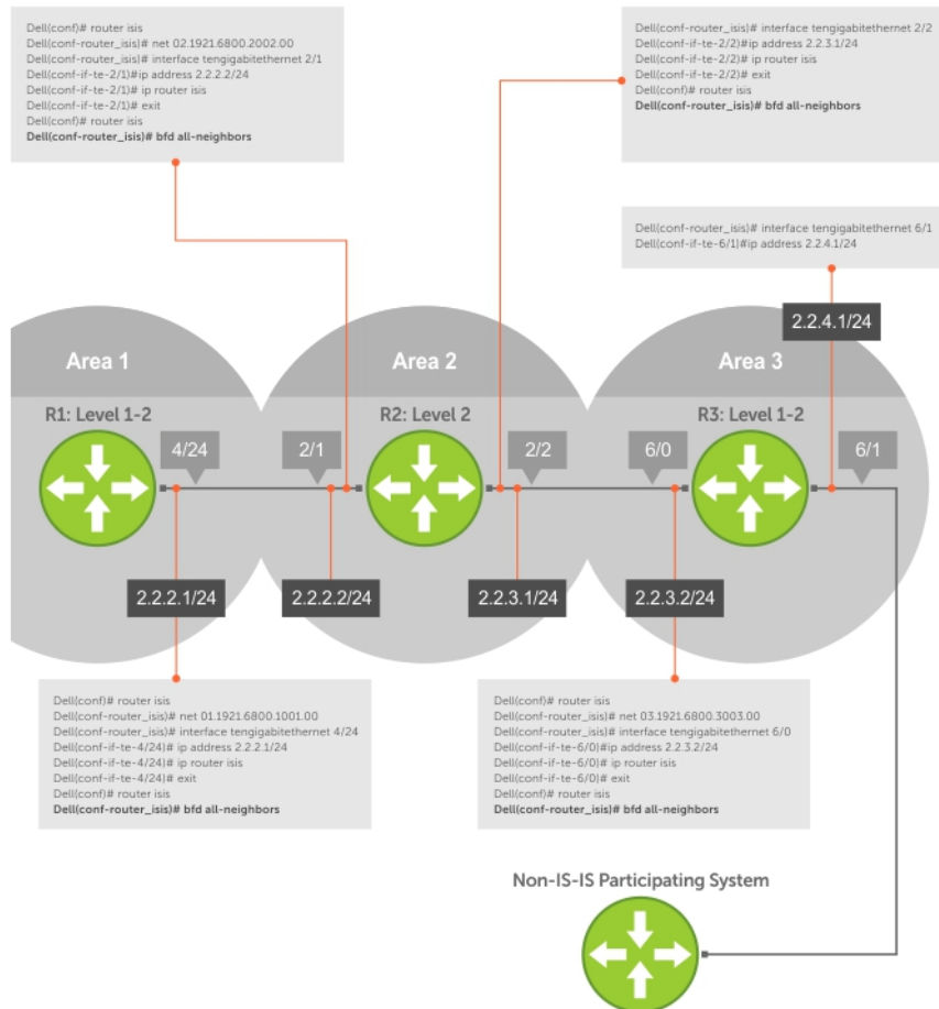
Figure 17. Establishing Sessions with IS-IS Neighbors
