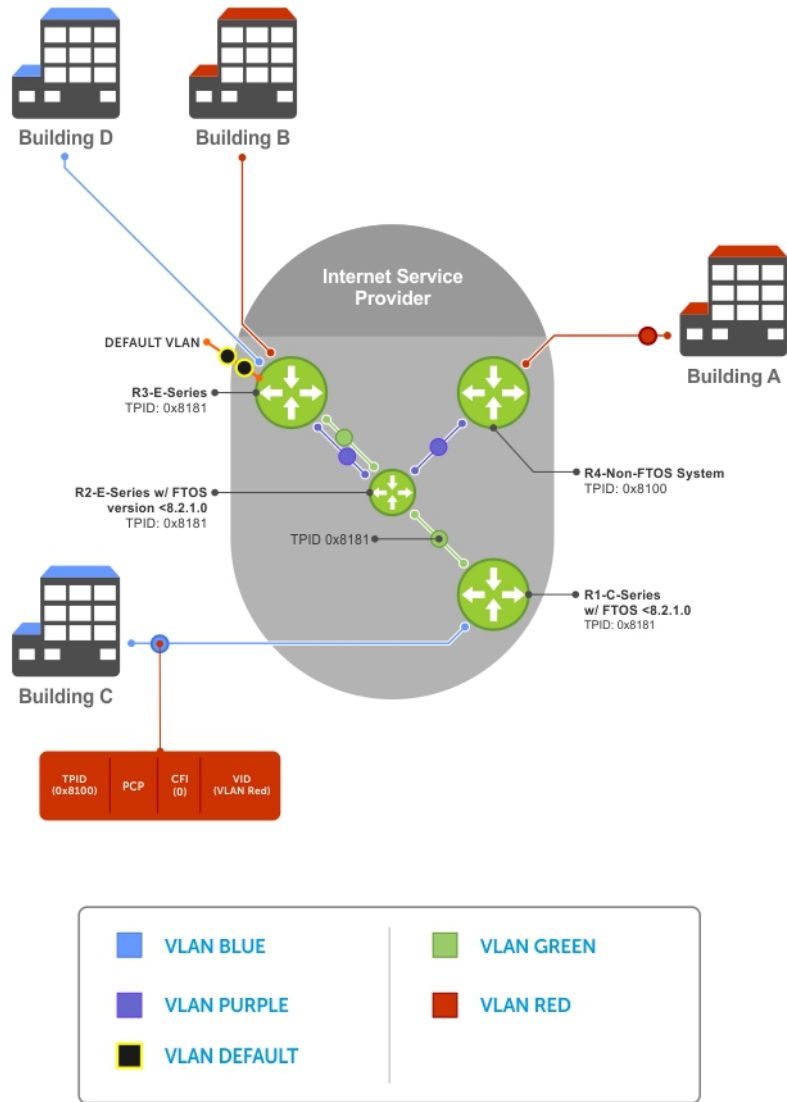
Figure 121. Single and Double-Tag First-byte TPID Match
