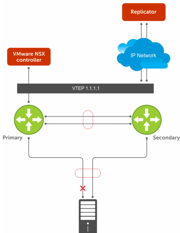
Figure 162. Controller-based VXLAN for VLT Providing Redundancy
