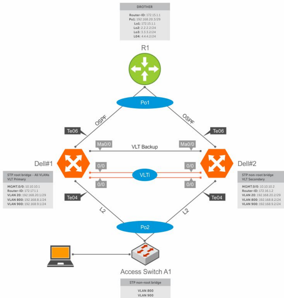
Figure 142. Peer Routing Configuration Example
