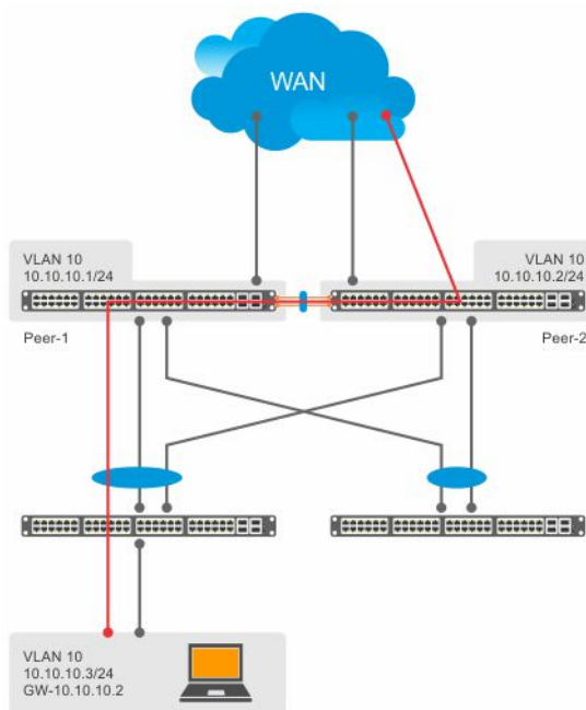
Figure 140. Packets without peer routing enabled
