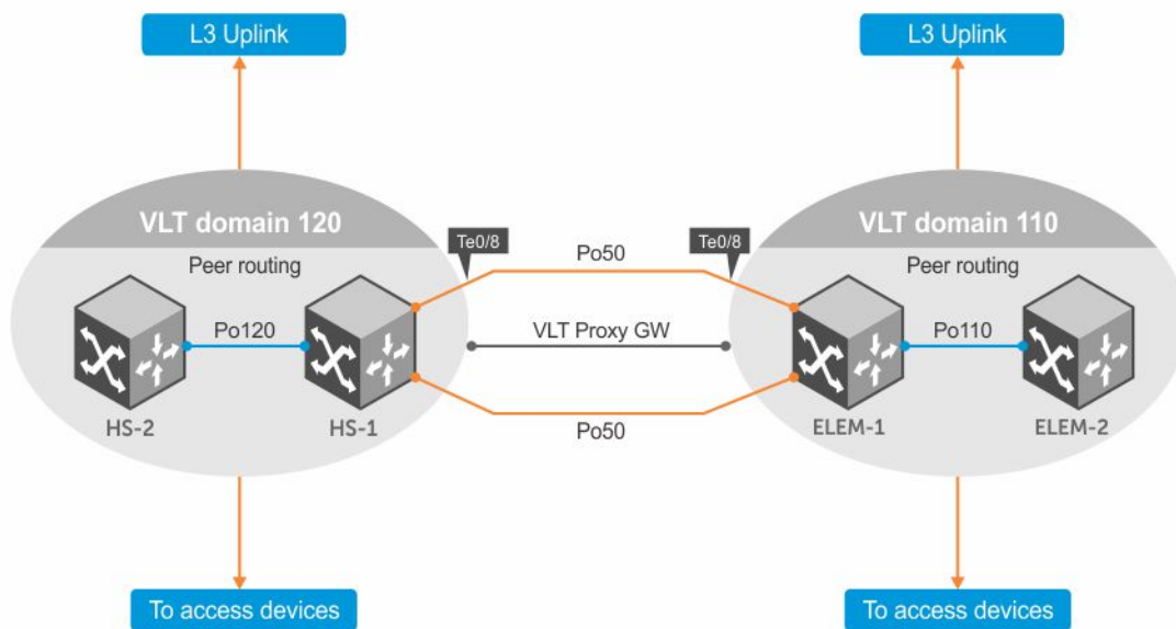
Figure 148. VLT Proxy Gateway Sample Topology
