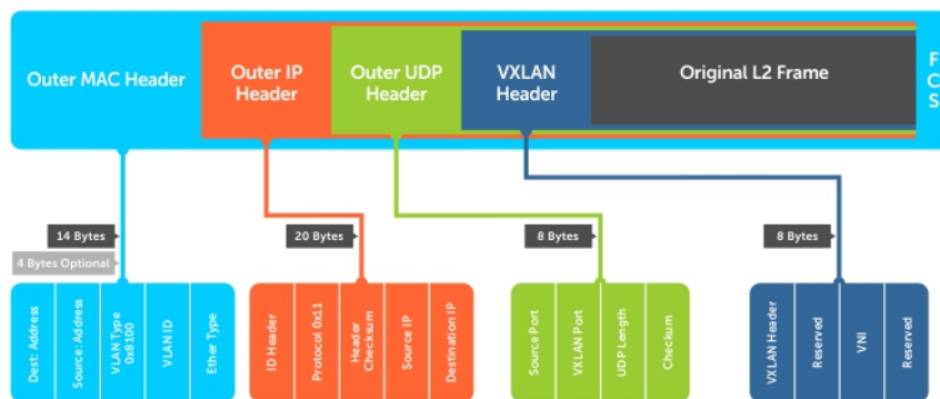
Figure 150. VXLAN Frame Format
