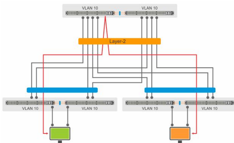
Figure 136. Layer-2 Traffic in VLT Domains
