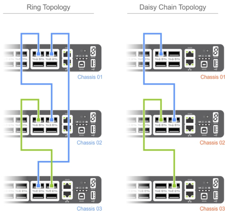
Figure 120. Supported Stacking Topologies
